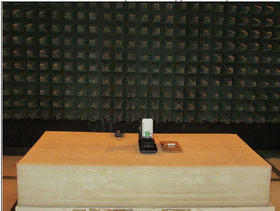
Radiated Emission (9kHz~30MHz) (Test Mode A)
