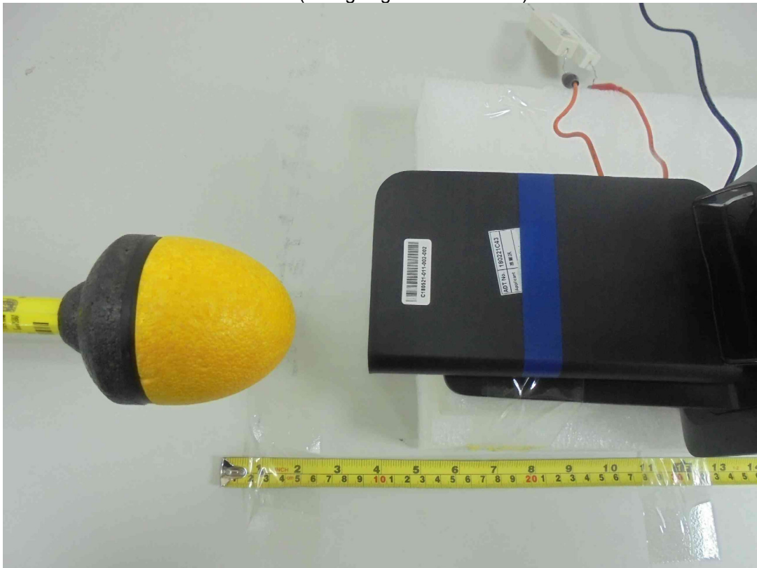
E-Field (Charging Mode with load)
