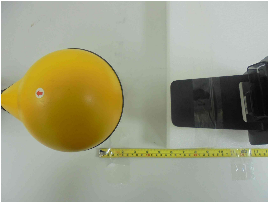
H-Field (Standby Mode)
