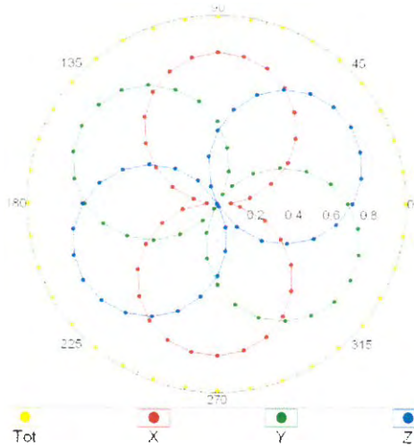
f=600 MHz,TEM
