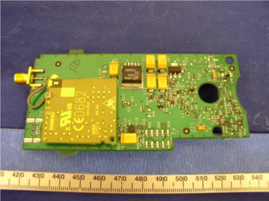
GPRS Interface Board Component View with GPRS Module
