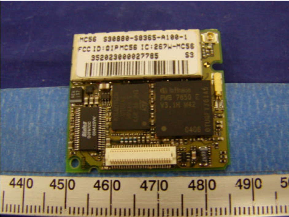
GPRS Module Component View
