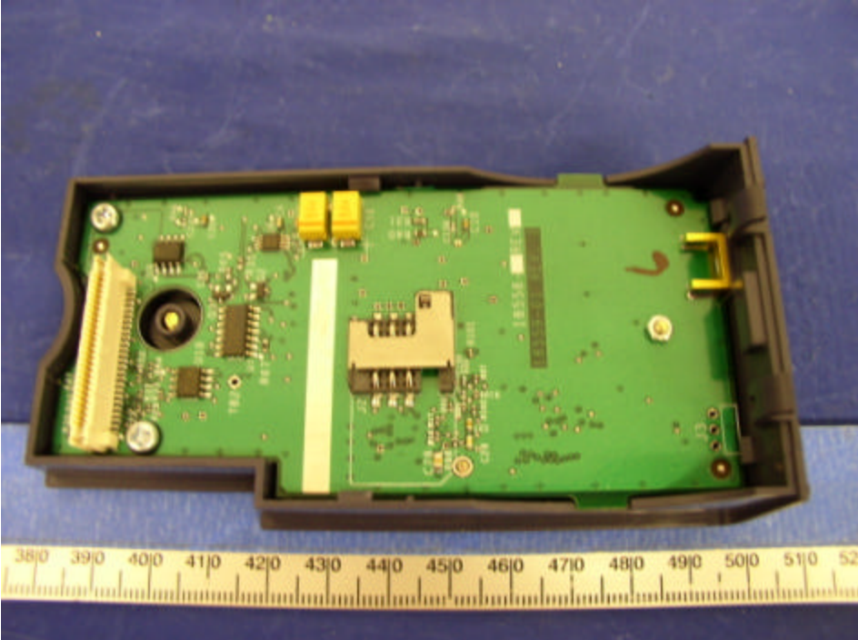
GPRS Interface Board View
