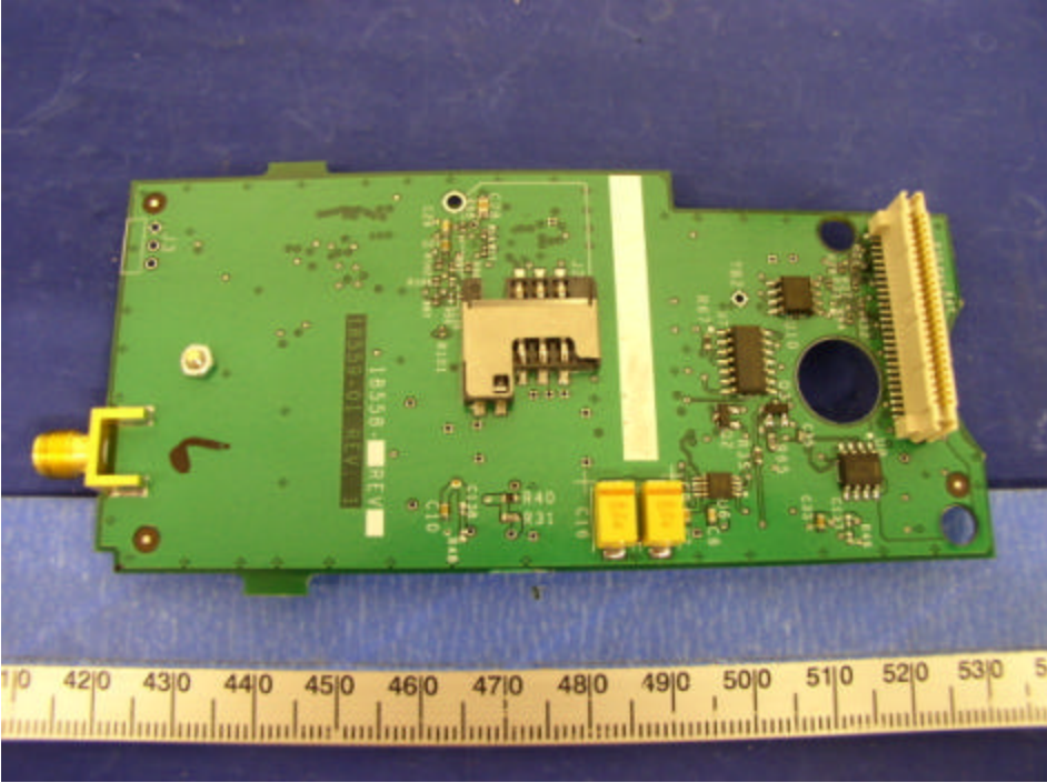
GPRS Interface Board Solder View
