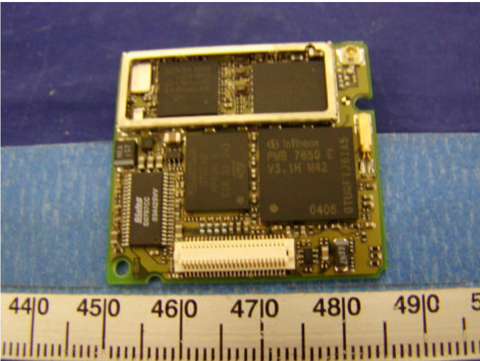
GPRS Module Component without Shielding View
