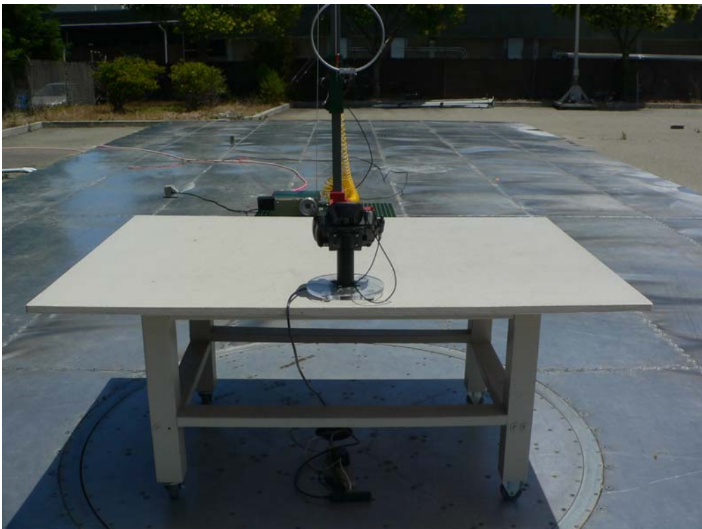
Radiated Emission – Rear View (Low Frequency)
