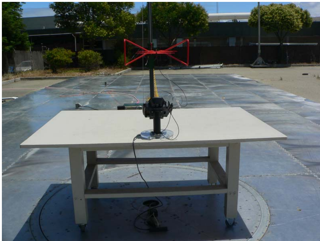
Radiated Emission – Rear View
