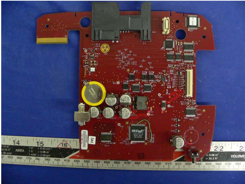
EUT 2 – Solder View
