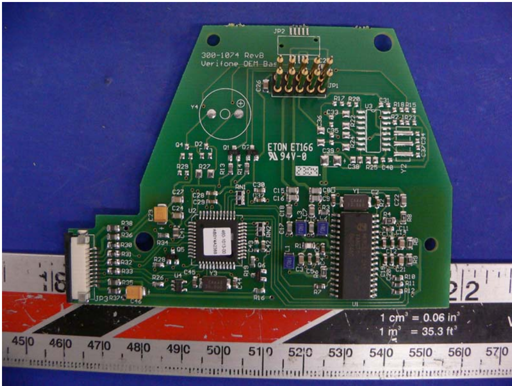
EUT 4 – Component View
