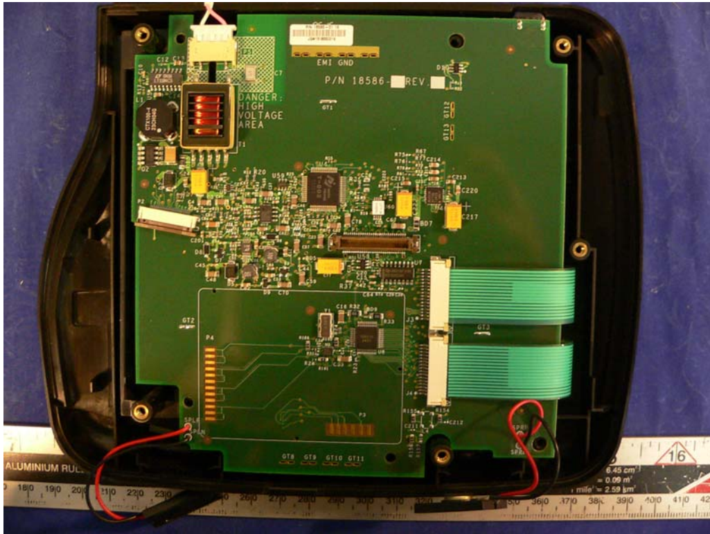
EUT 2 – Cover Off View
