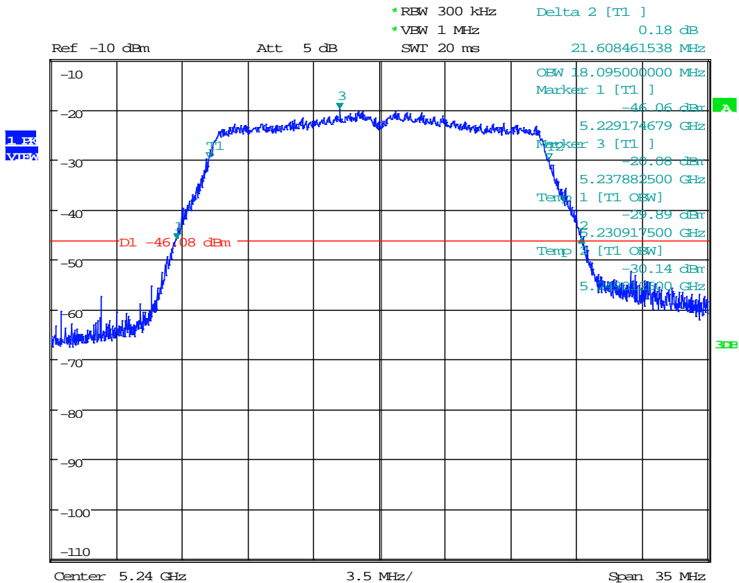
Plot 1. 6 802.11n 20MHz, 5240MHz
