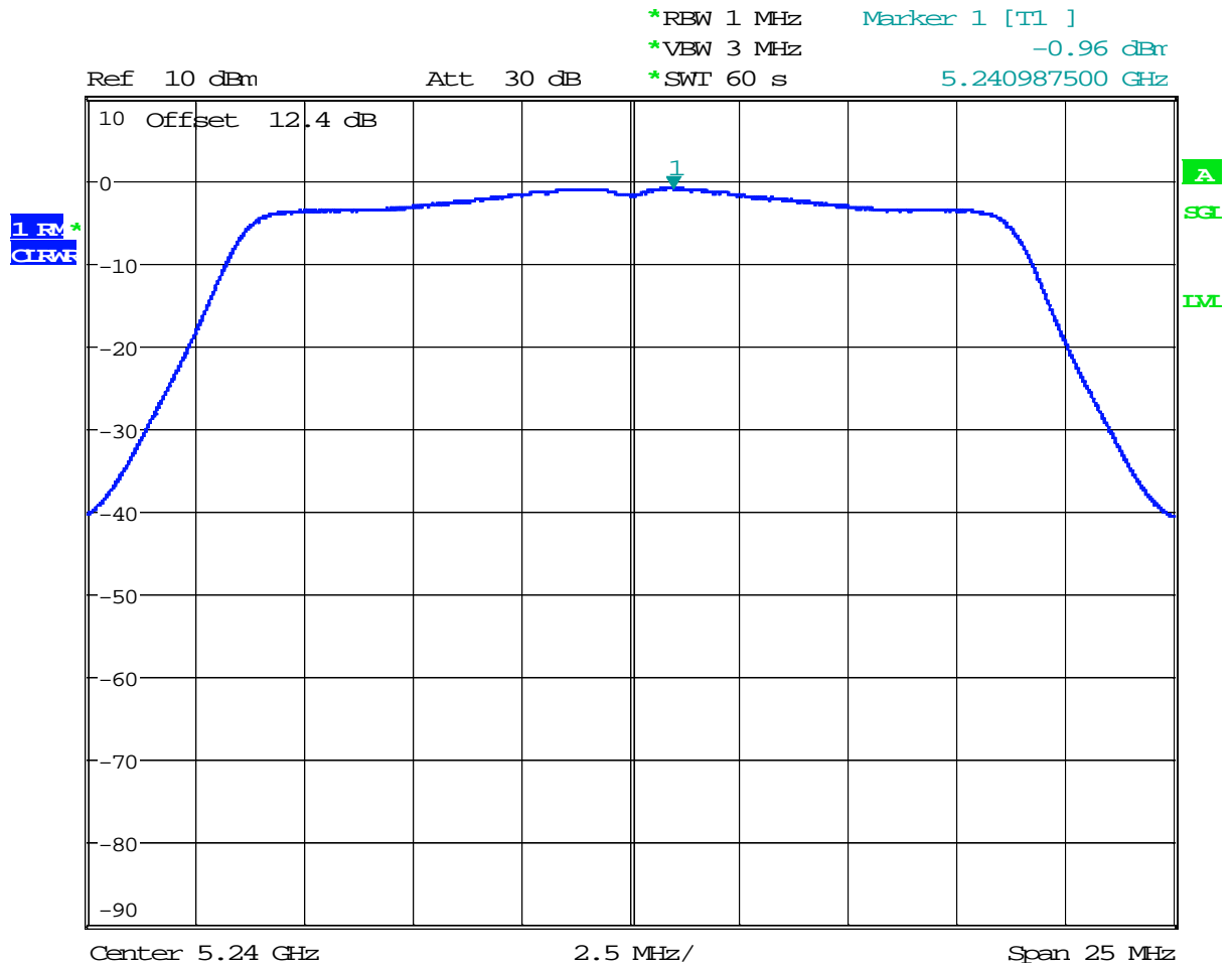
Plot 3. 14 802.11n 20MHz, 5240MHz
