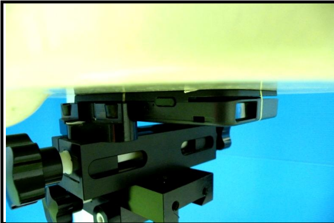
Front Face of EUT with 0 cm Gap
