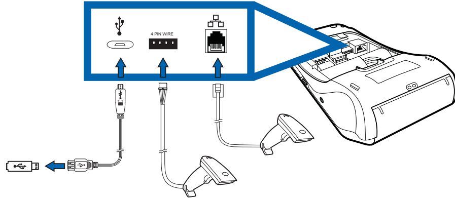
Figure 8 Connection Ports
