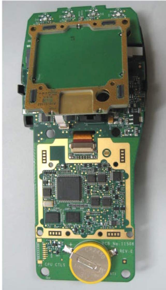
Photograph No. 3 PINpad 1000se CTLS / Qx1000 main PCB and Grid-Perimeter PCB, 180° rolled
