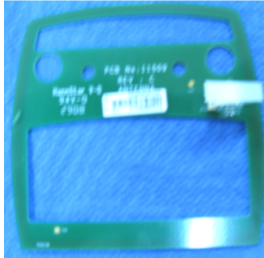
Photograph No. 6 PINpad 1000se CTL5 / Qx1000 loop antenna PCB second sideview
