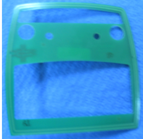
Photograph No. 5 PINpad 1000se CTLS / Qx1000 loop antenna PCB front view
