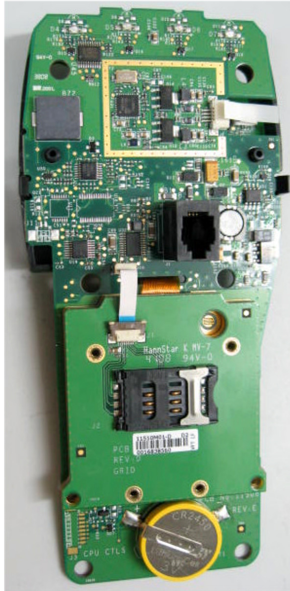
Photograph No. 2 PINpad 1000se CTL5 / Qx1000 main PCB and Grid-Perimeter PCB
