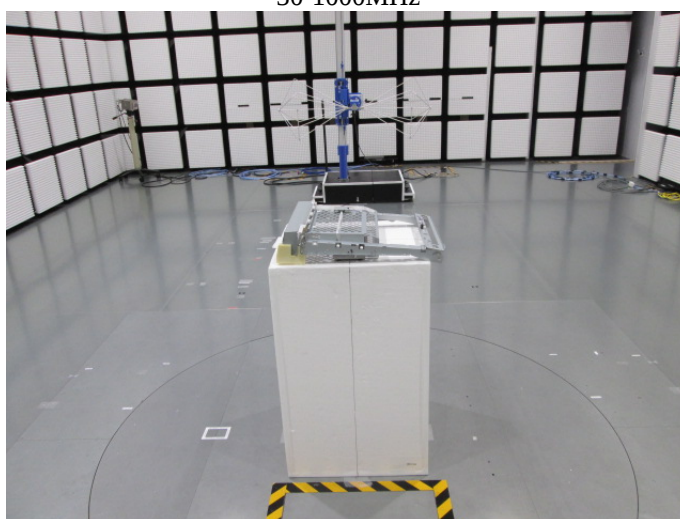
Rear 30-1000MHz
