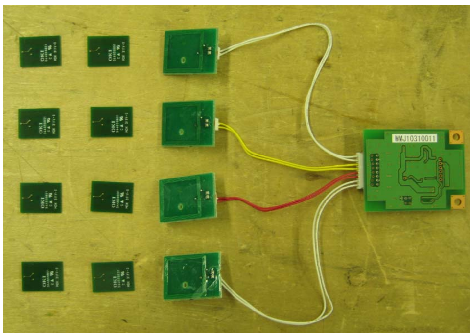
Inside view of Internal Circuit with antennas <Rear>
