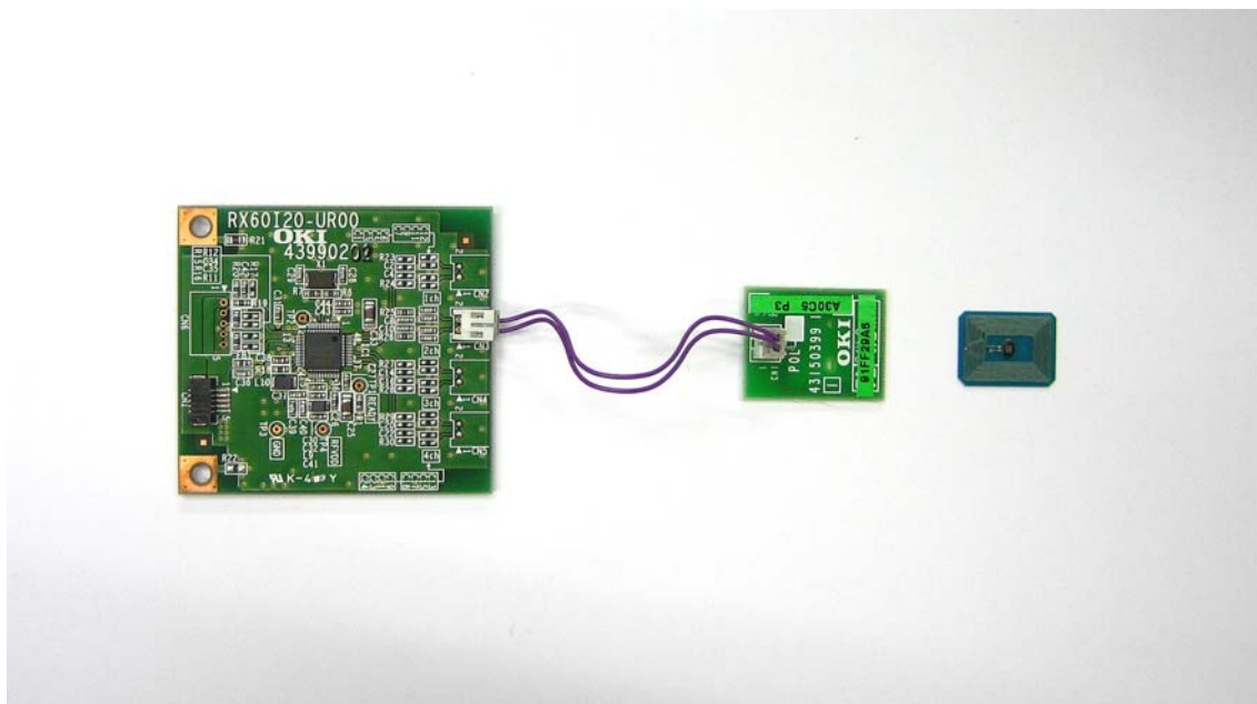
Inside view of Internal Circuit with antennas <Front>
