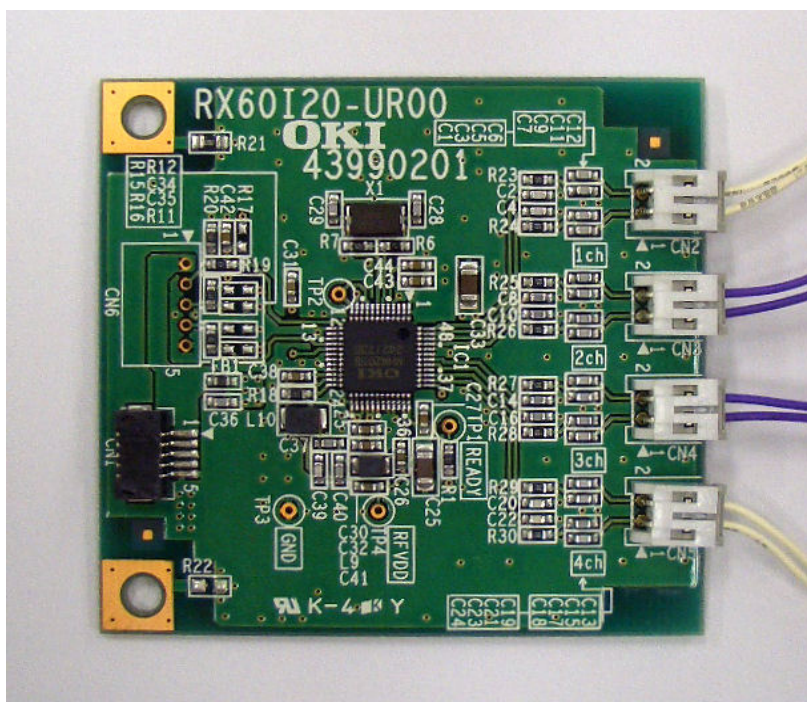
Inside view of Internal circuit <Front>
