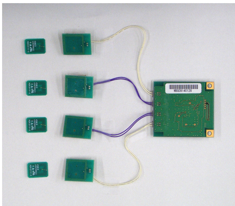
Inside view of Internal Circuit with antennas <Rear>
