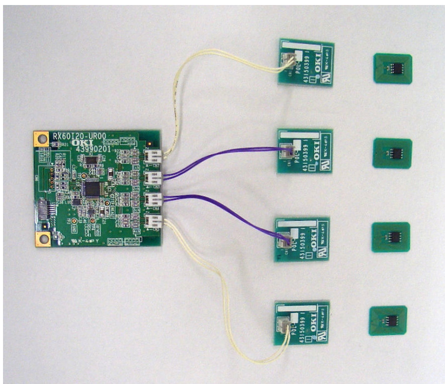
Inside view of Internal Circuit with antennas <Front>
