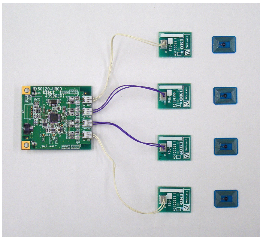
Inside view of Internal Circuit with antennas <Front>
