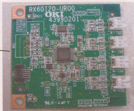
RF Module without shielding (Photo 2)
