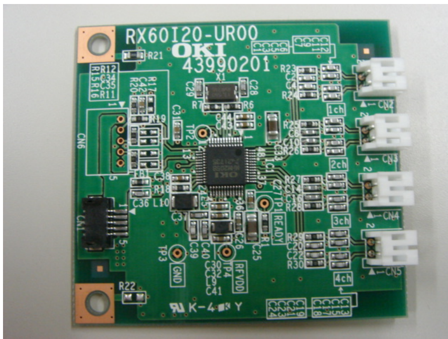
Inside View of Internal Circuit<Front>
