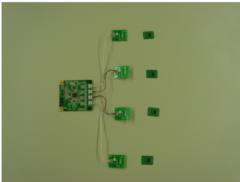
Inside View of Internal Circuit with antennas<Front>
