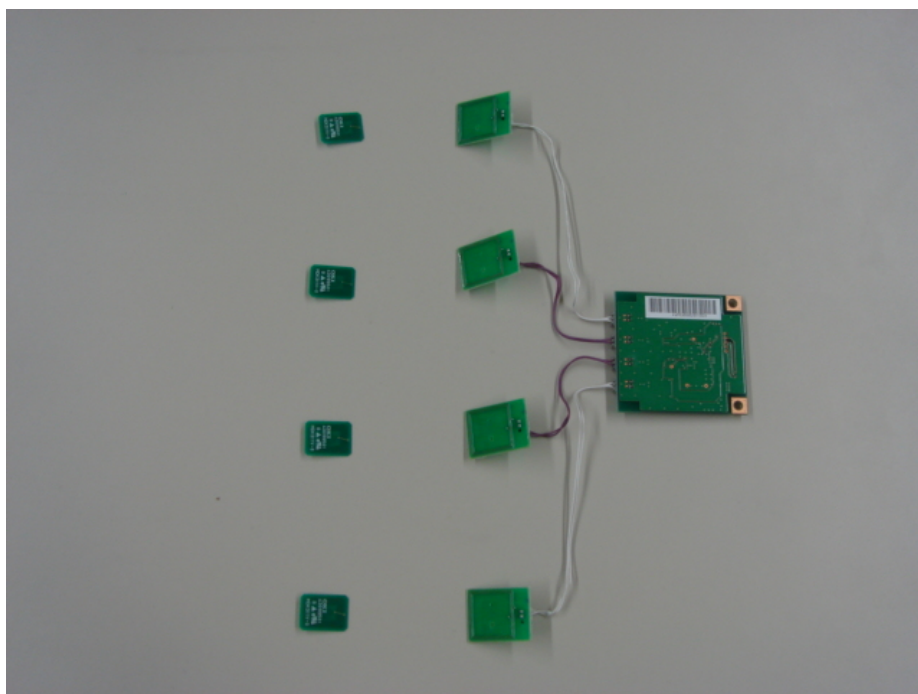
Inside View of Internal Circuit with antennas<Rear>
