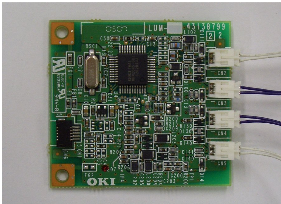
Inside view of Internal circuit <Front>
