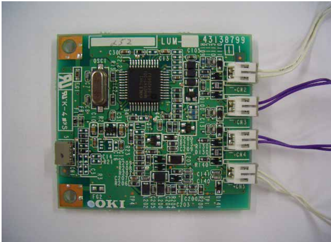
Inside view of Internal circuit <Front>
