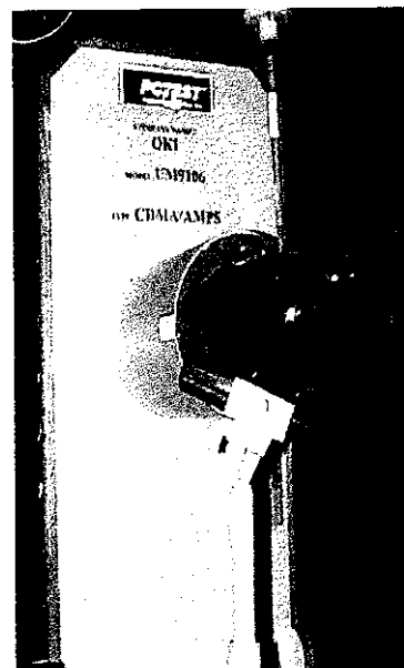
Figure 1. SAR Test Set-up
