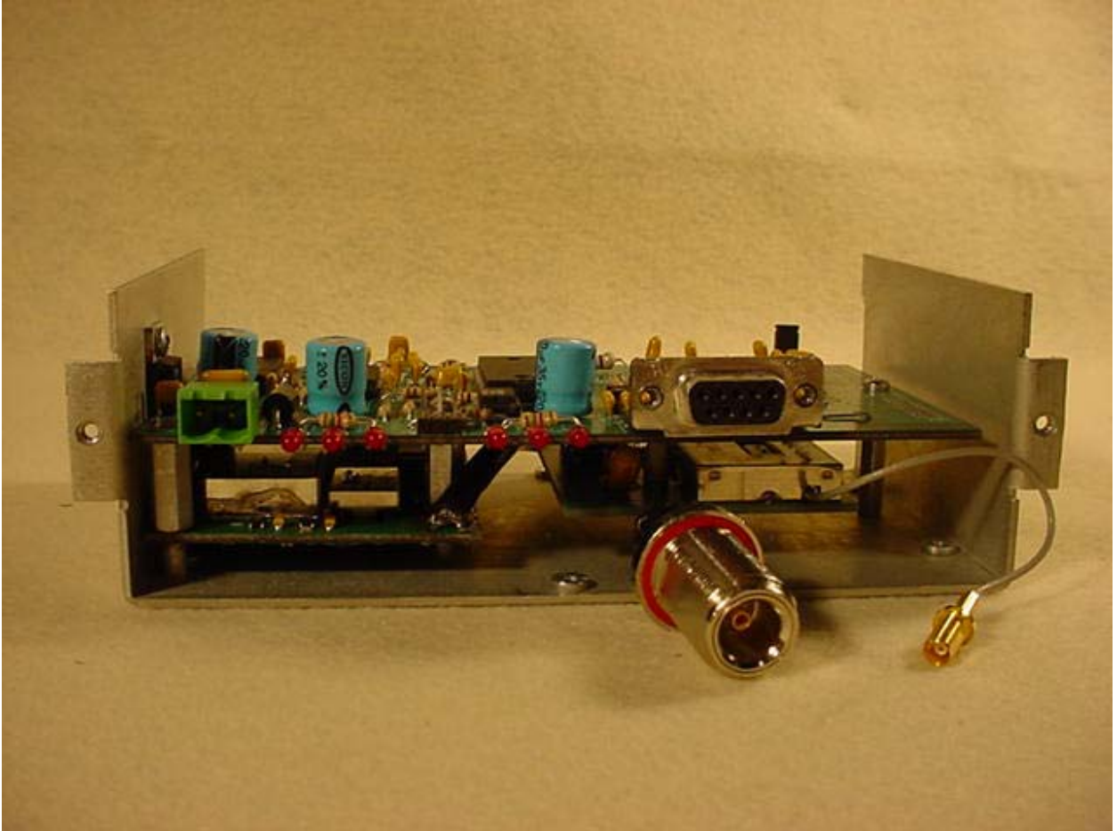
Figure 8: Mounted – Front View
