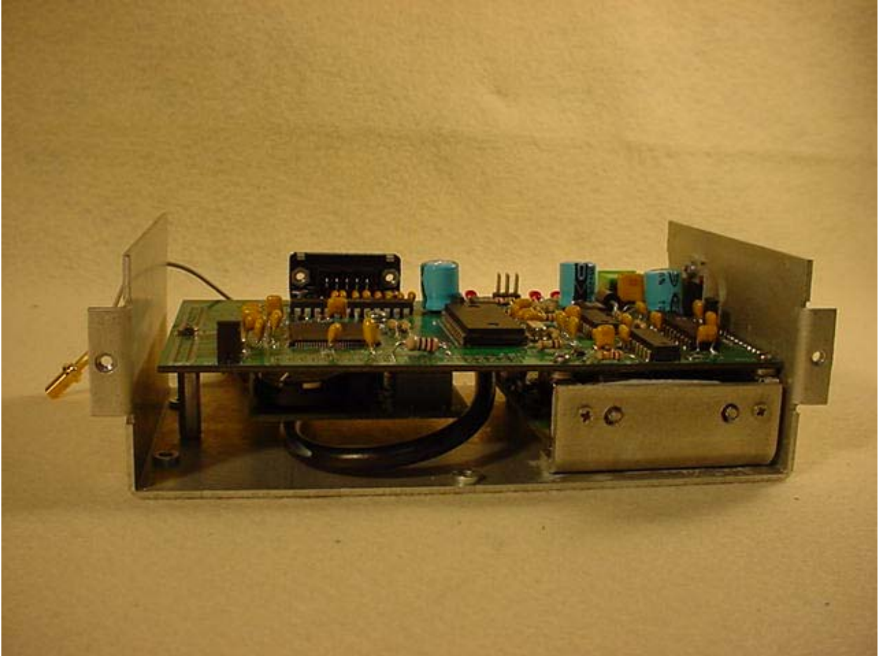
Figure 9: Mounted – Rear View
