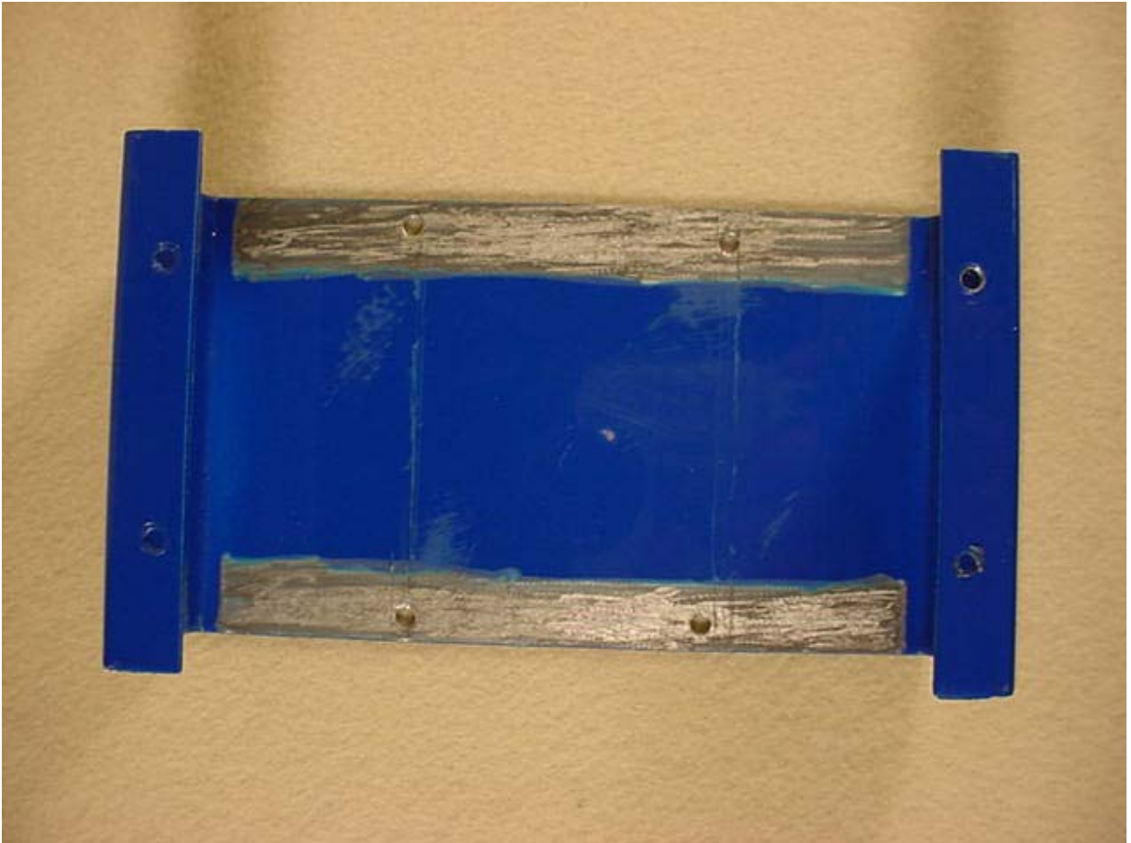
Figure 5: Outer Shell – Top View
