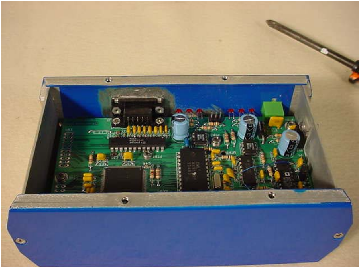
Figure 3: Internal – Top-rear Angled View
