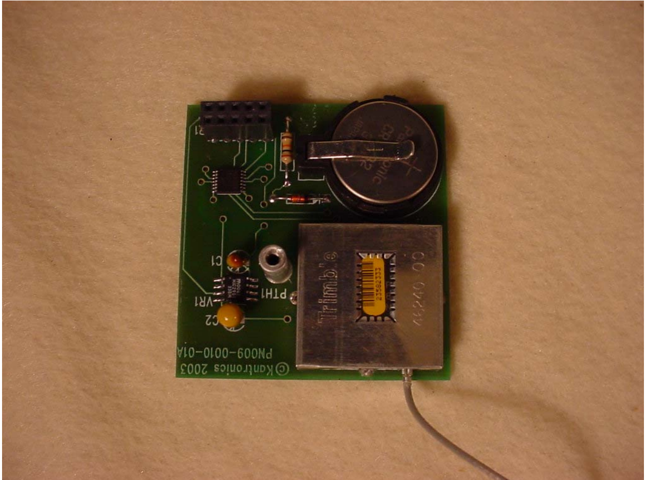
Figure 5: GPS Transmitter – Top View
