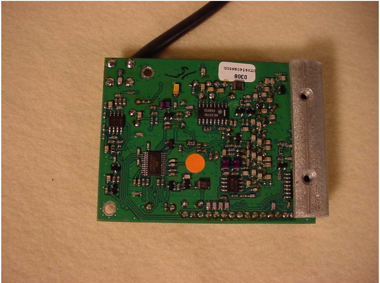
Figure 4: RF Transmitter – Bottom View
