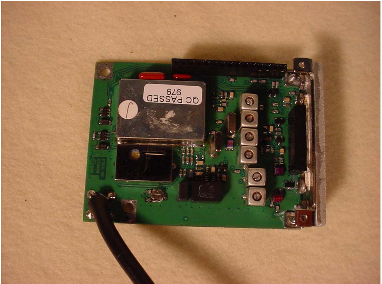
Figure 3: RF Transmitter – Top View
