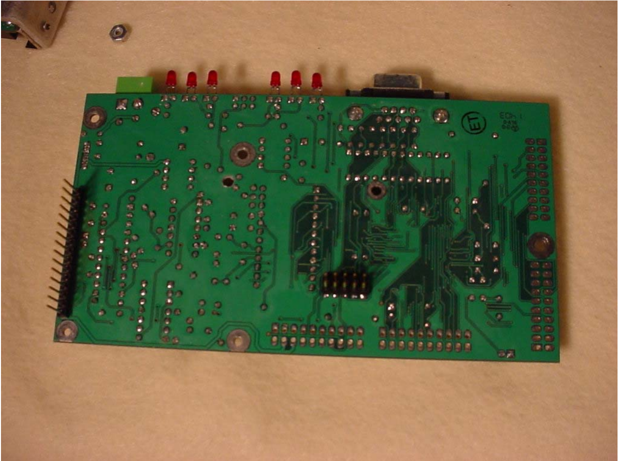
Figure 2: Control Board – Bottom View
