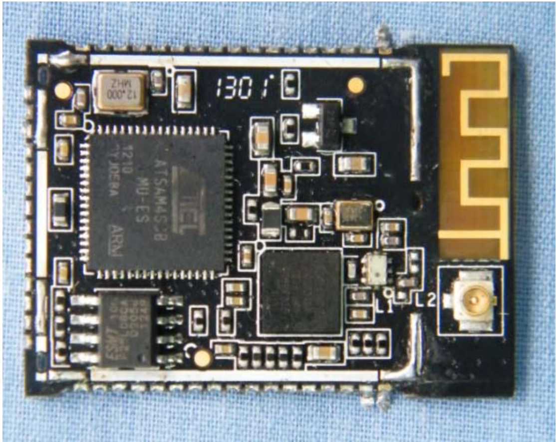
AZY-HF-LPB Internal photo
