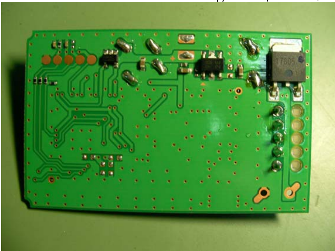
Figure 6 General Appearance (RF Module, Back View)
