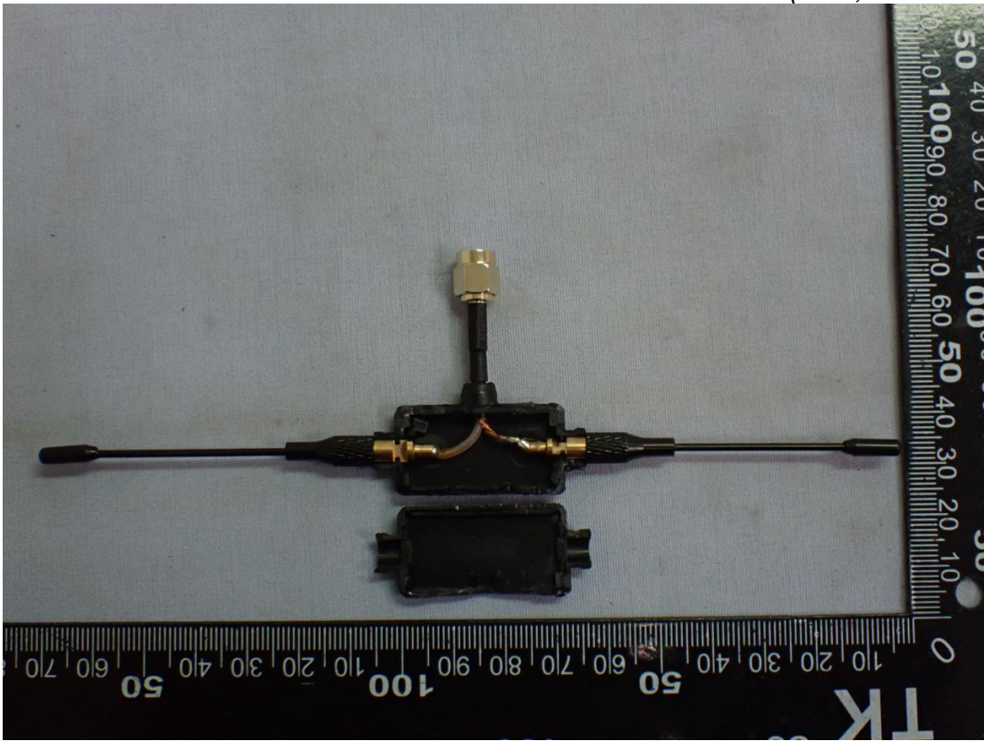
Figure 8 Internal View (ANT, Removed Cover)
