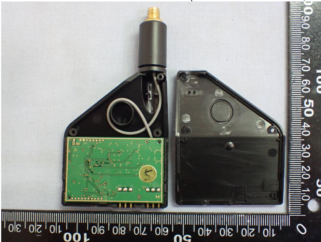
Internal View (Removed Cover/RF Board, Back View)
