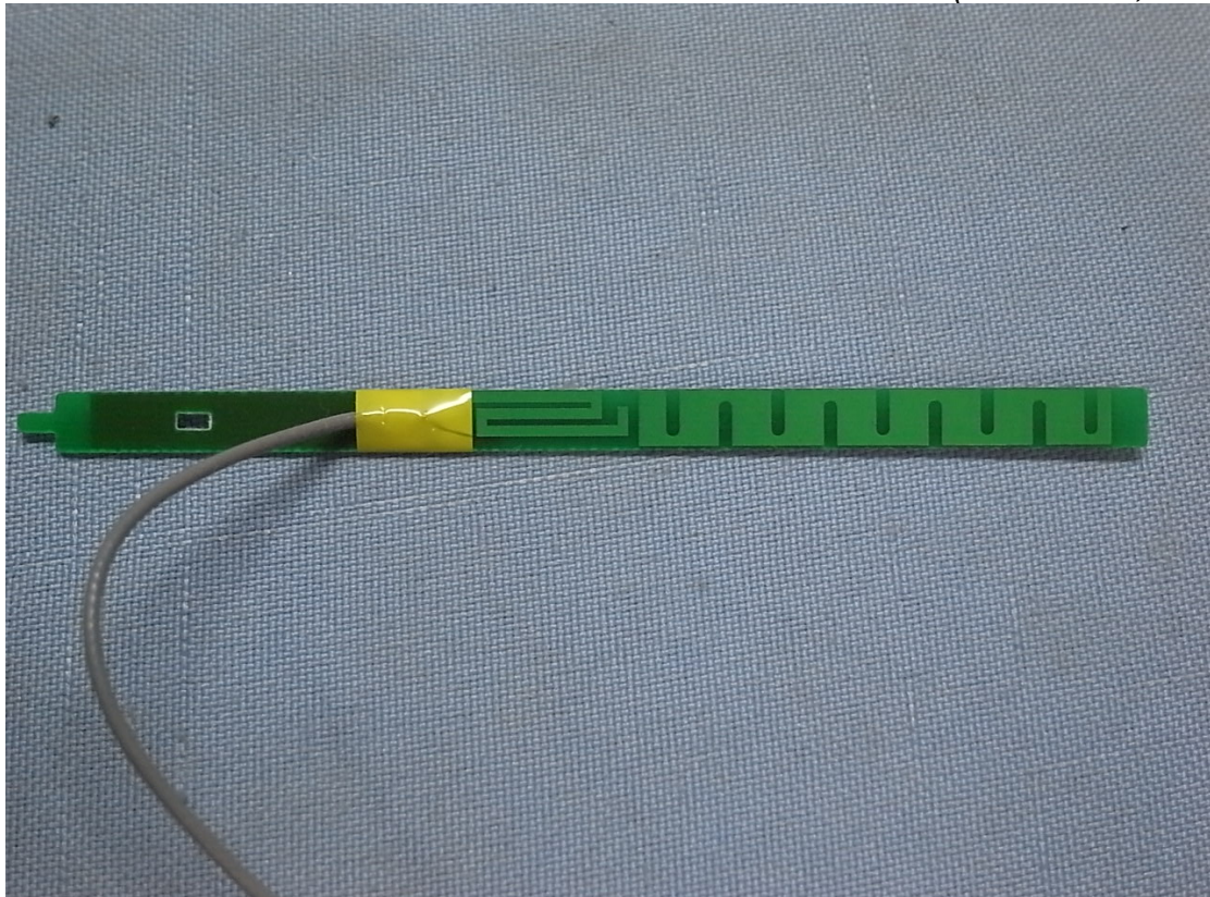
Figure 11 Internal View (ANT Board, Front View)
