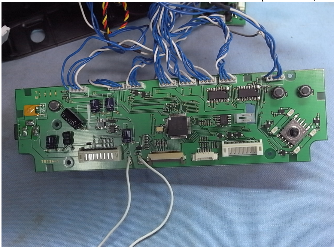
Figure 6 Internal View (Main Board, Front View)
