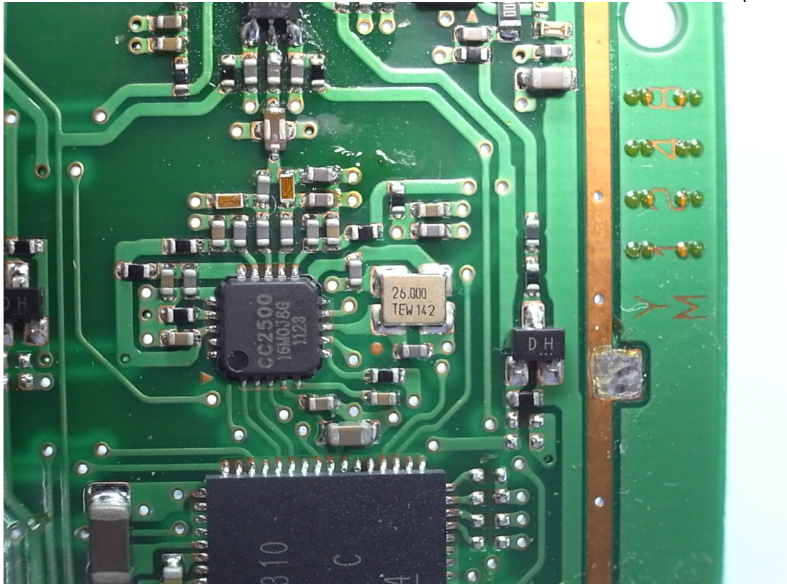
Figure 9 Internal View (RF Module)
