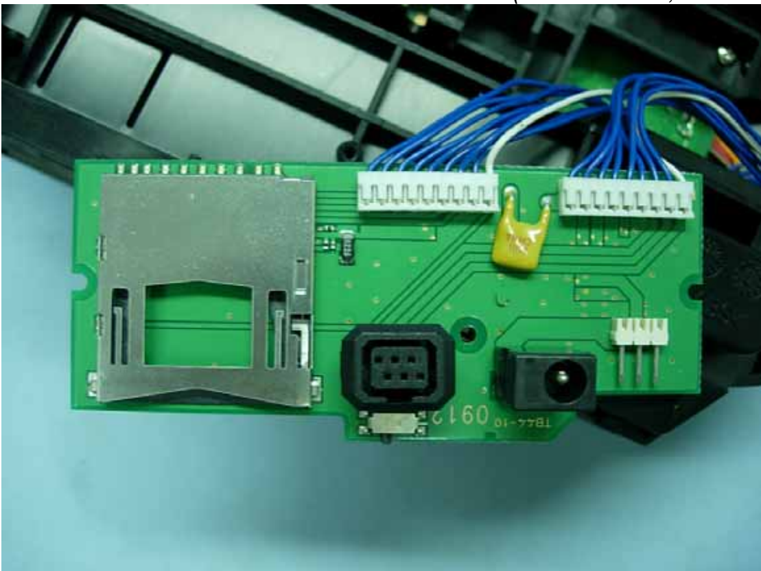
Figure 11 Internal View (TB44-10 Board, Front View)
