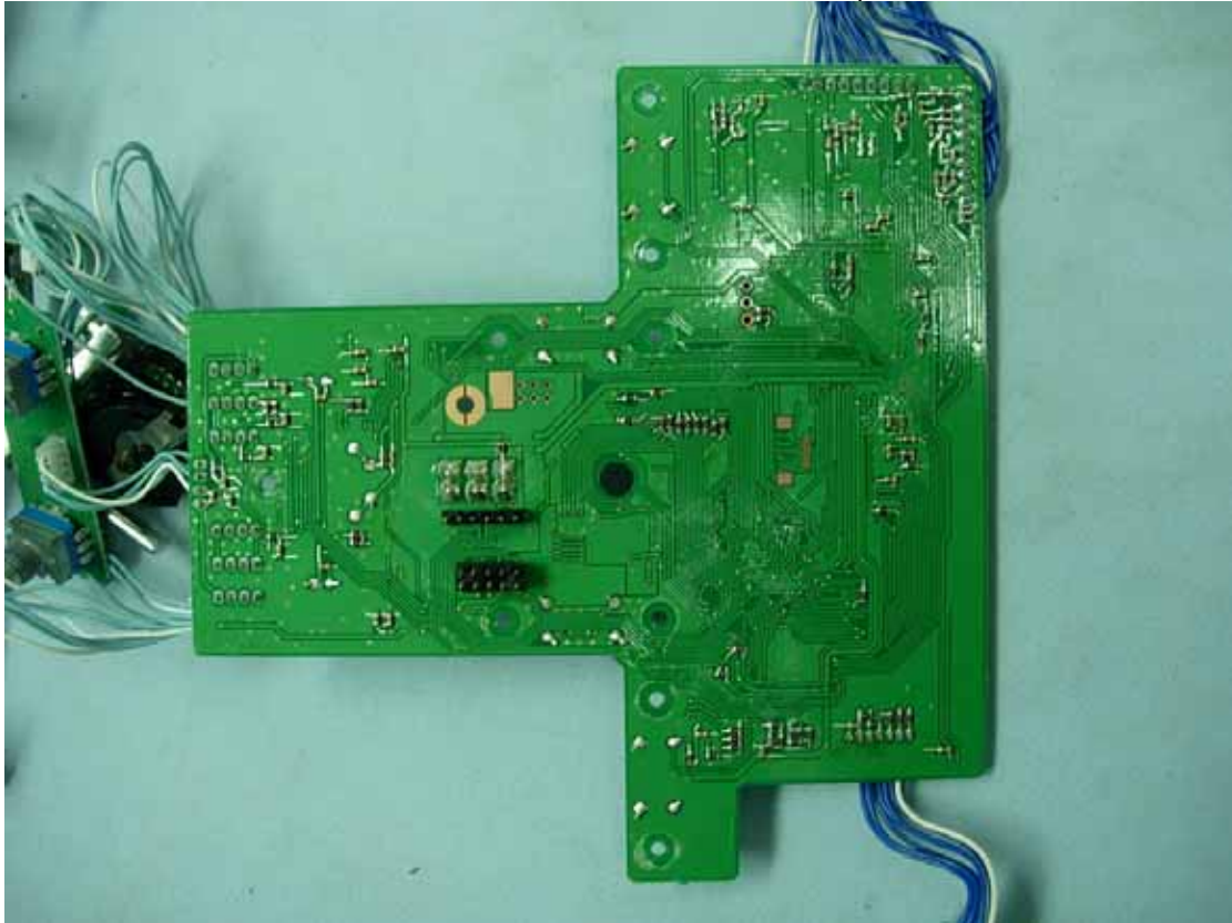
Figure 26 Internal View (TB44-1 Board, Back View)
