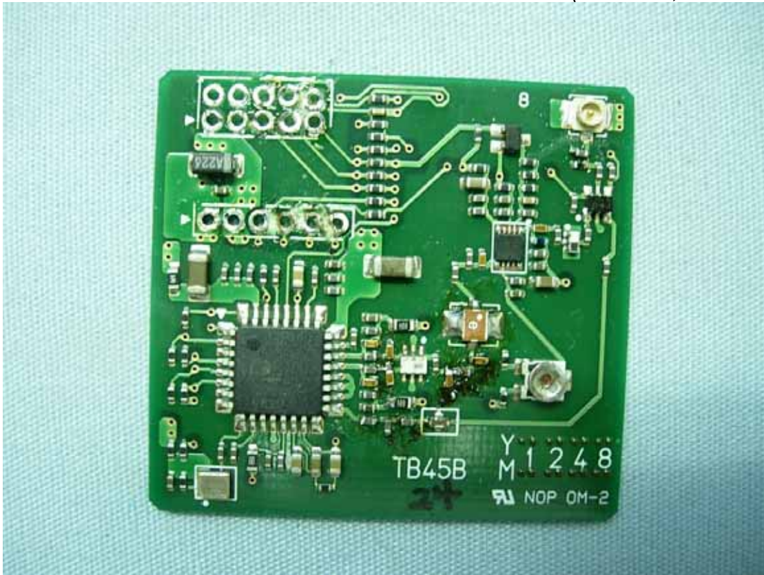
Figure 14 Internal View (RF Board, Front View)
