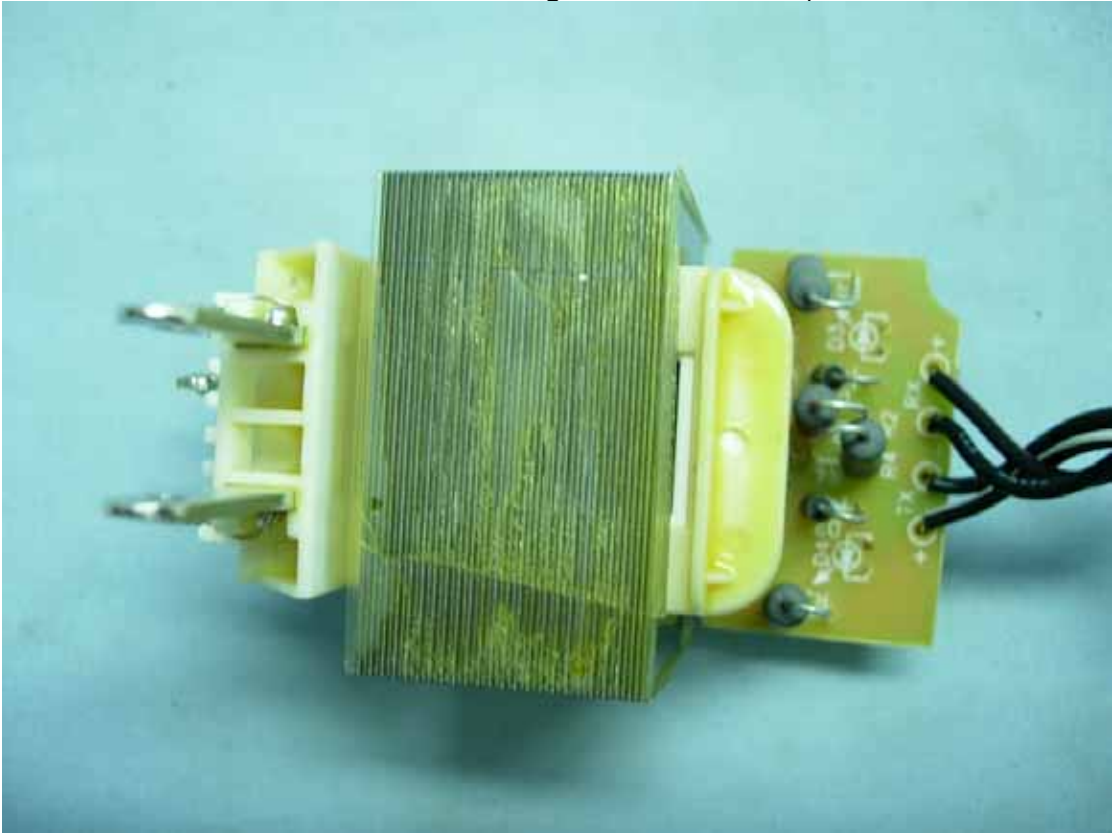
Figure 28 Ni-MH Charger, Internal View (PCB Board, Front View)
