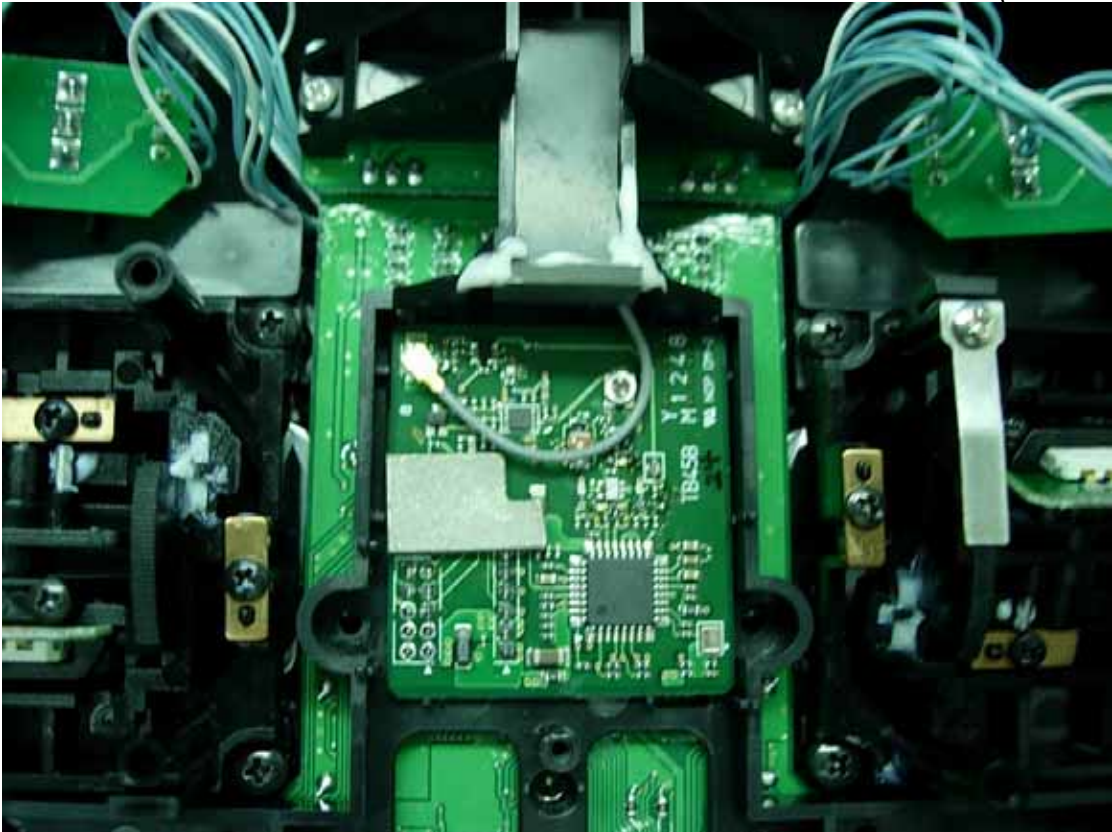
Figure 13 Internal View (RF Board)
