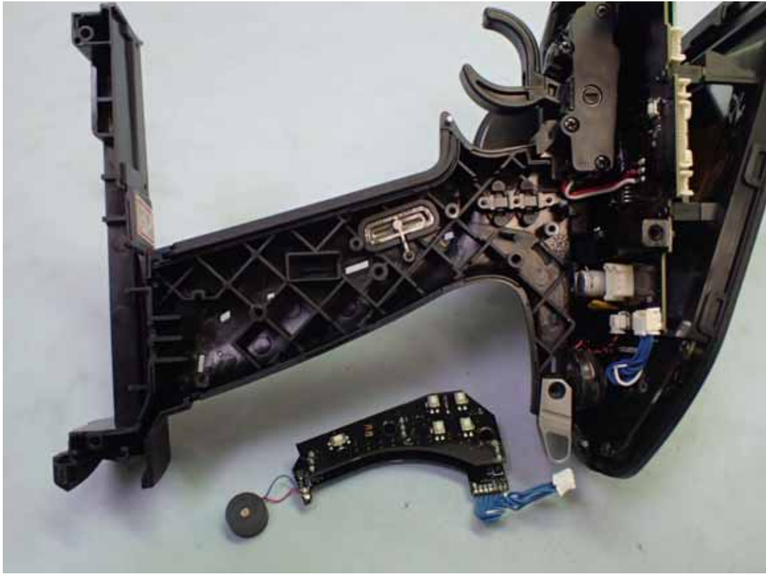
Figure 22 Internal View
