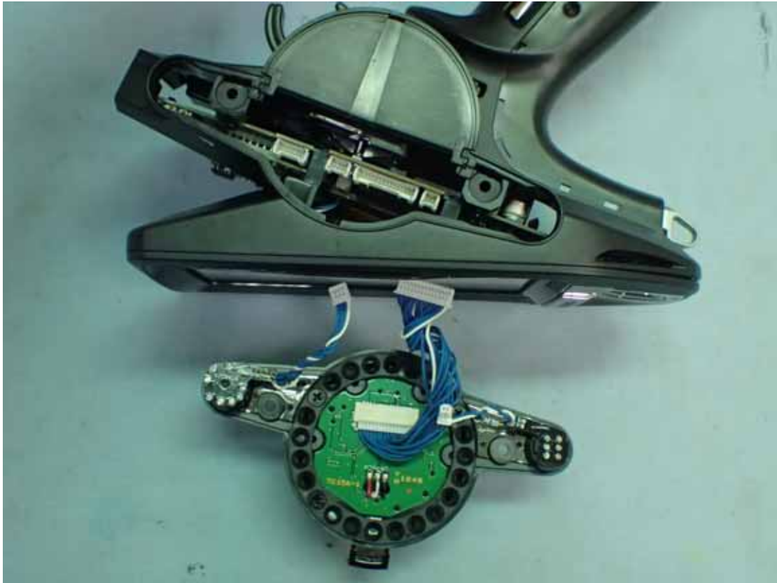
Figure 27 Internal View
