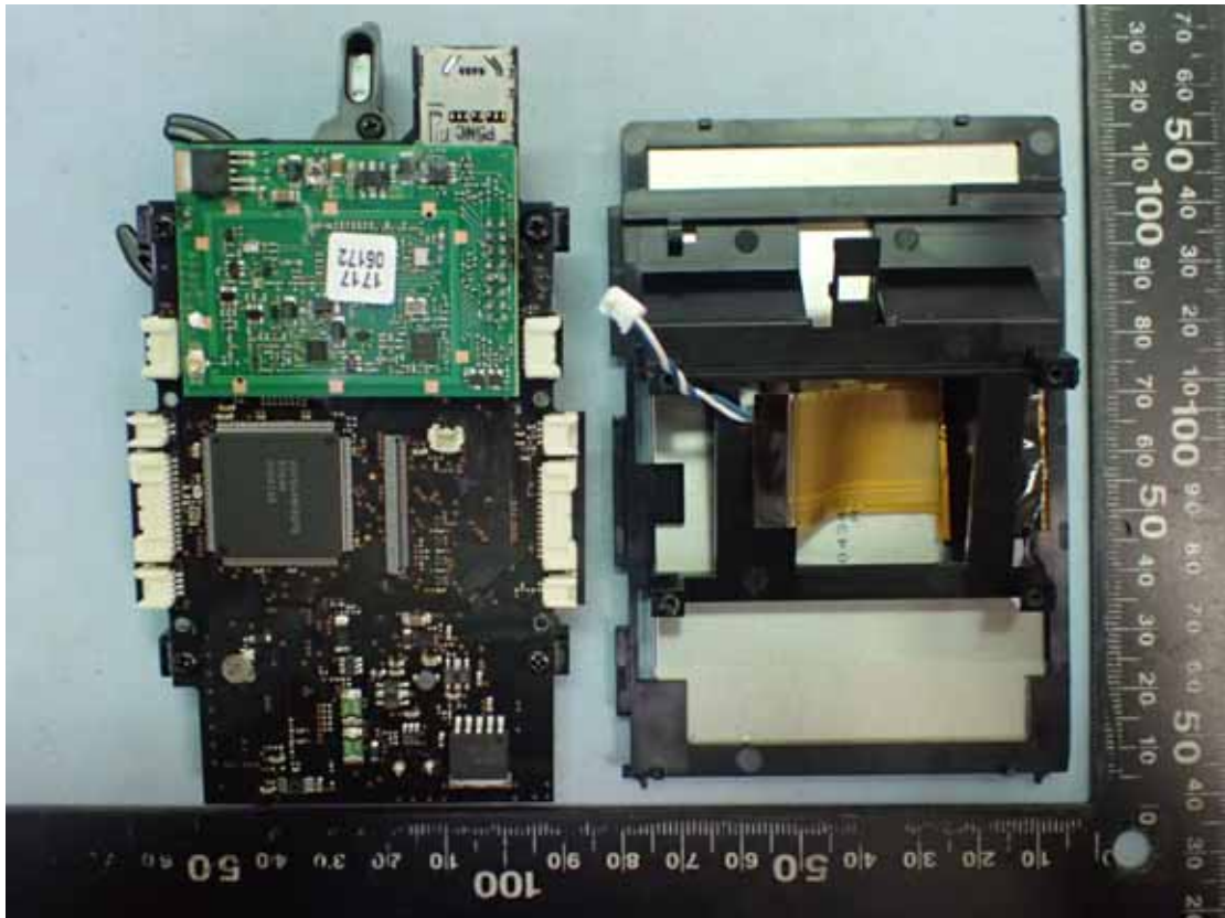
Figure 36 Internal View
