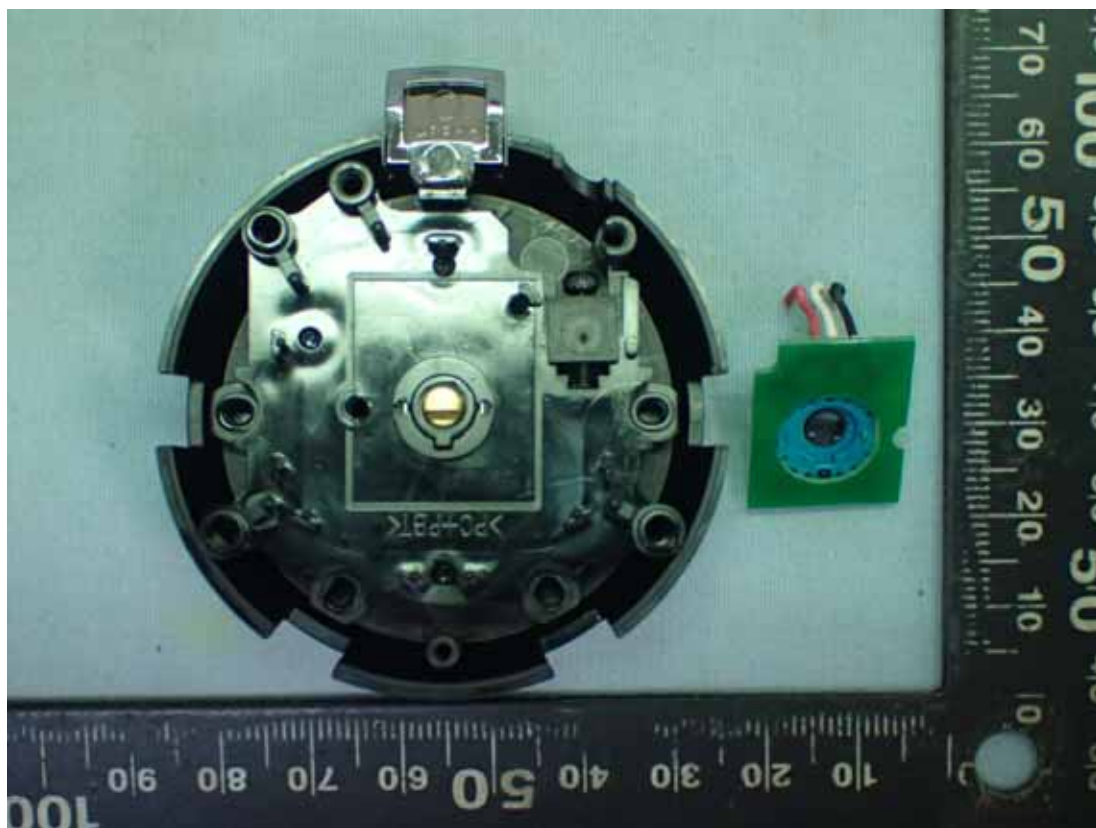
Figure 30 Internal View
