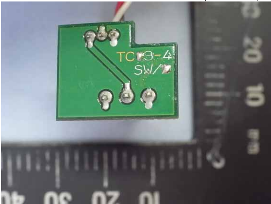
Figure 14 Internal View (TC03-4 Board, Back View)
