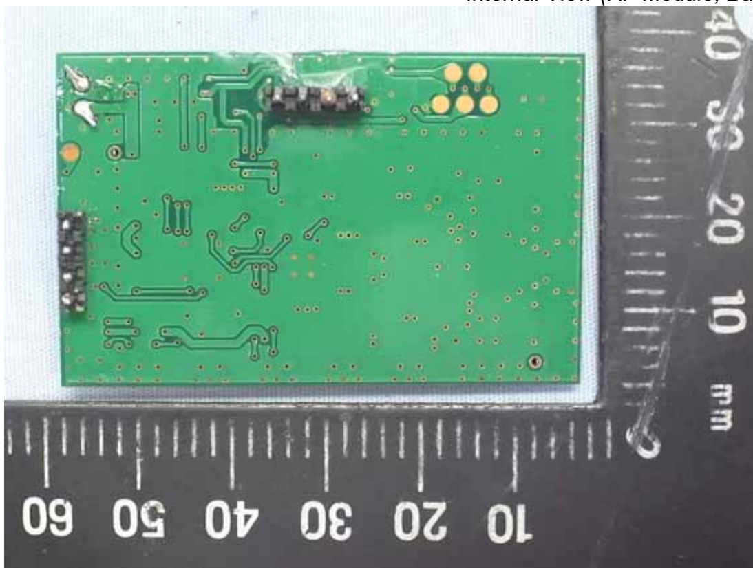
Figure 19 Internal View (RF Module, Back View)
