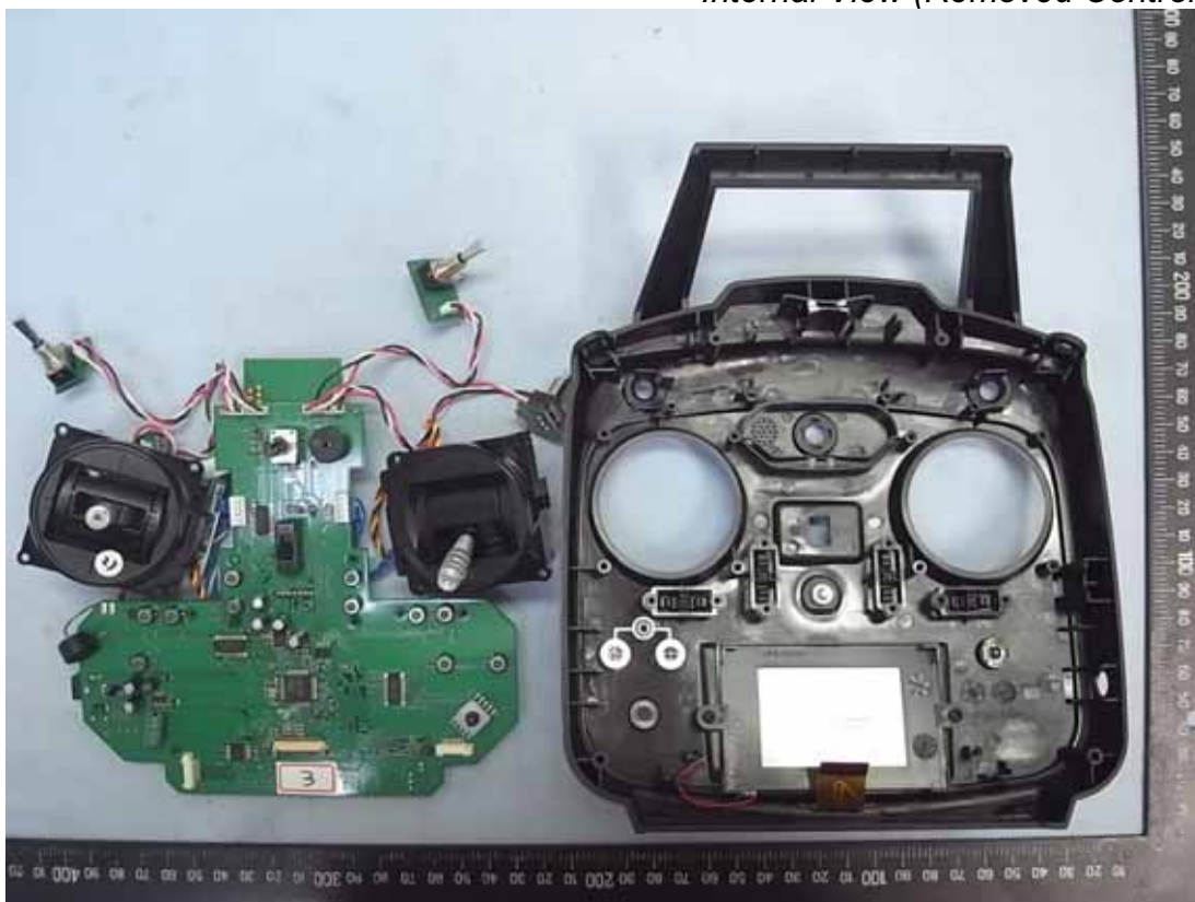
Figure 10 Internal View (Removed Control Boards)
