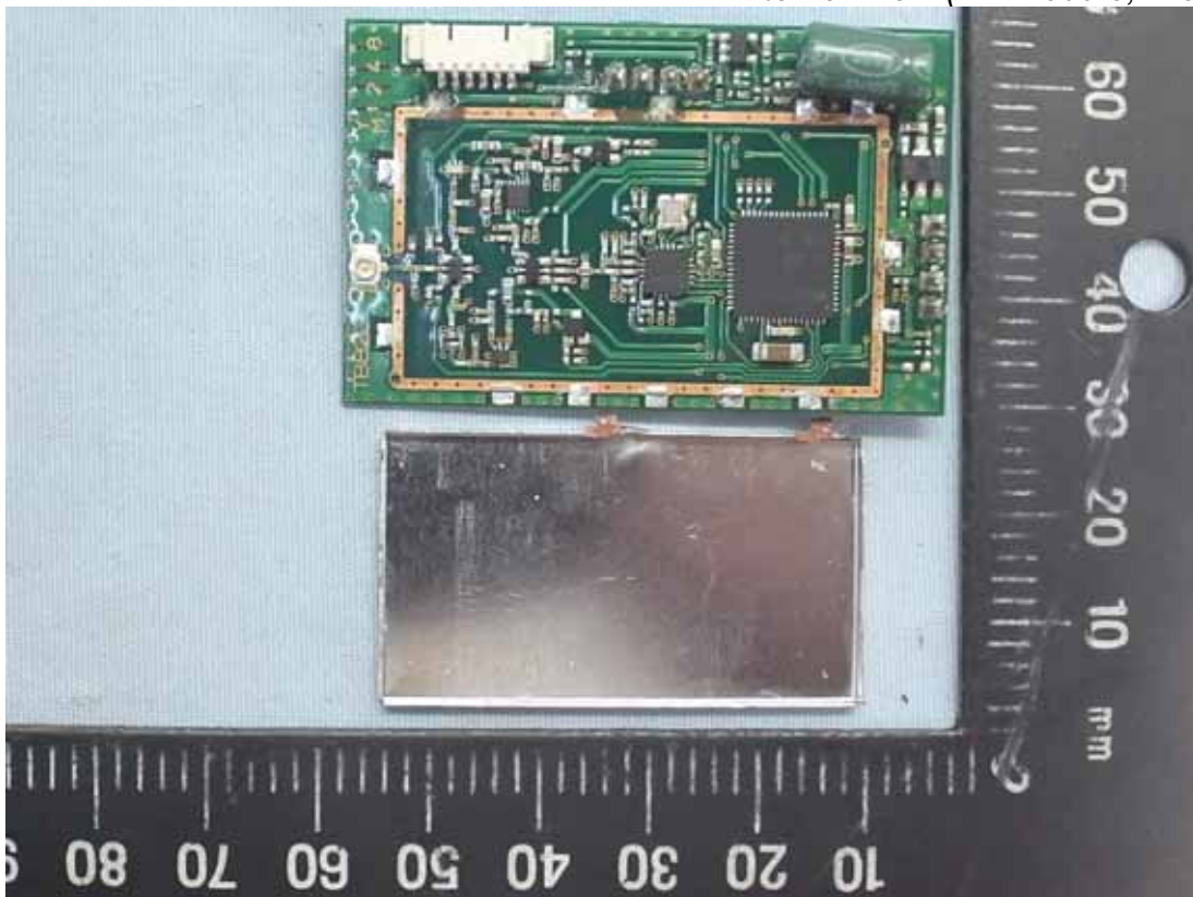
Figure 18 Internal View (RF Module, Front View)
