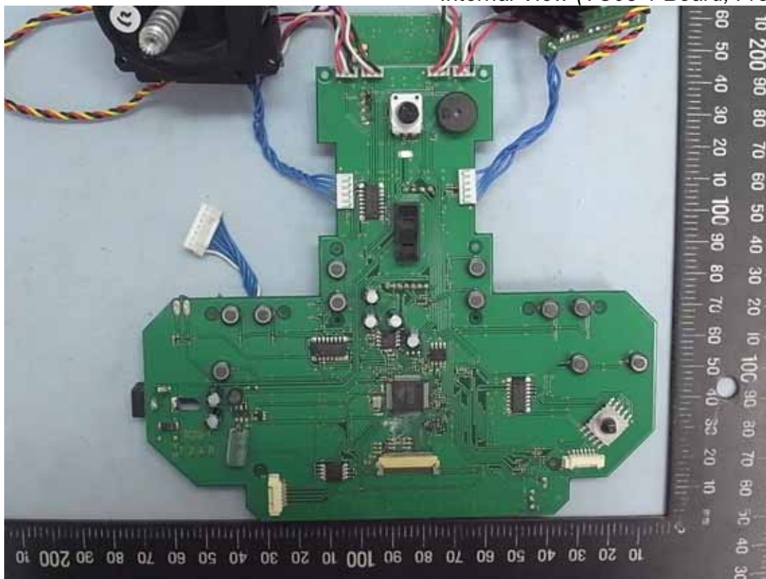
Figure 15 Internal View (TC03-1 Board, Front View)
