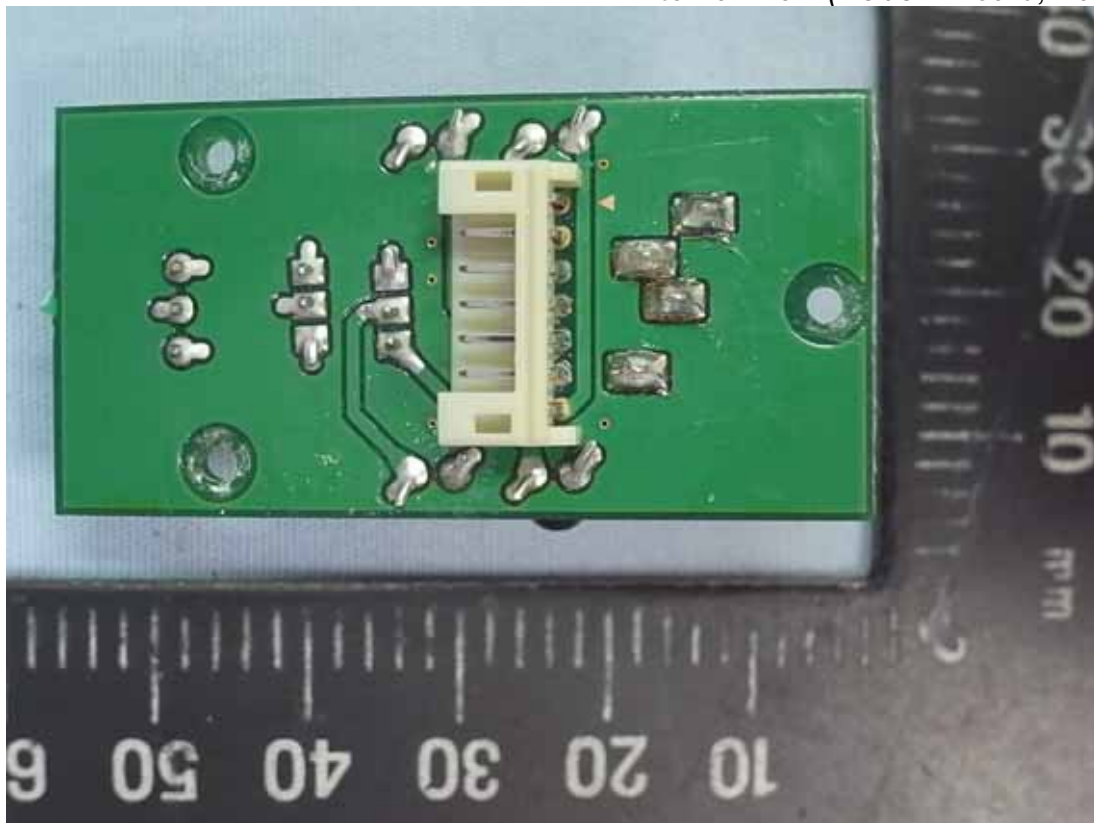
Figure 6 Internal View (TC03-2 Board, Back View)
