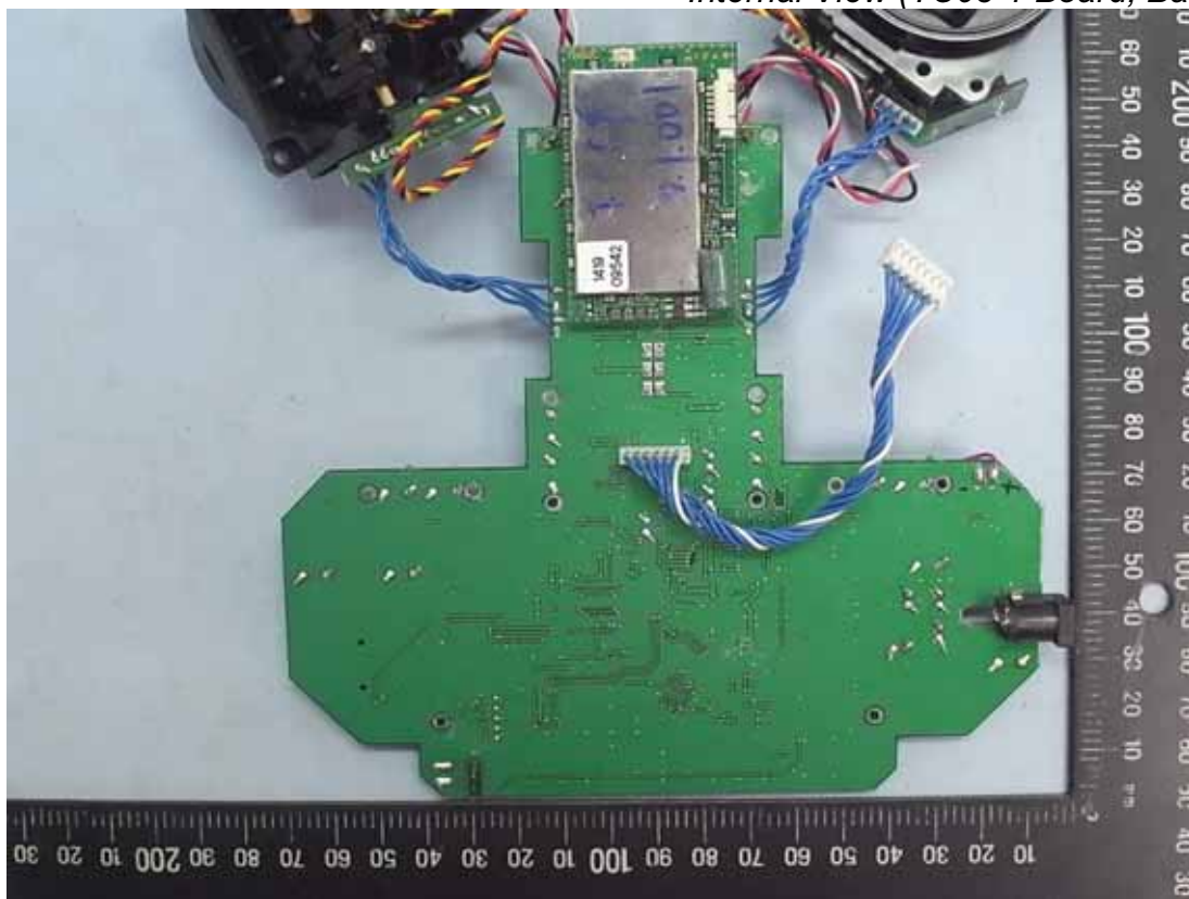
Figure 16 Internal View (TC03-1 Board, Back View)
