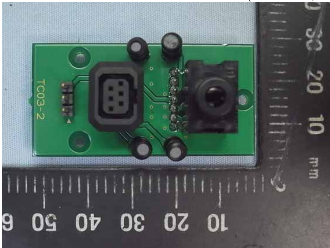
Figure 5 Internal View (TC03-2 Board, Front View)
