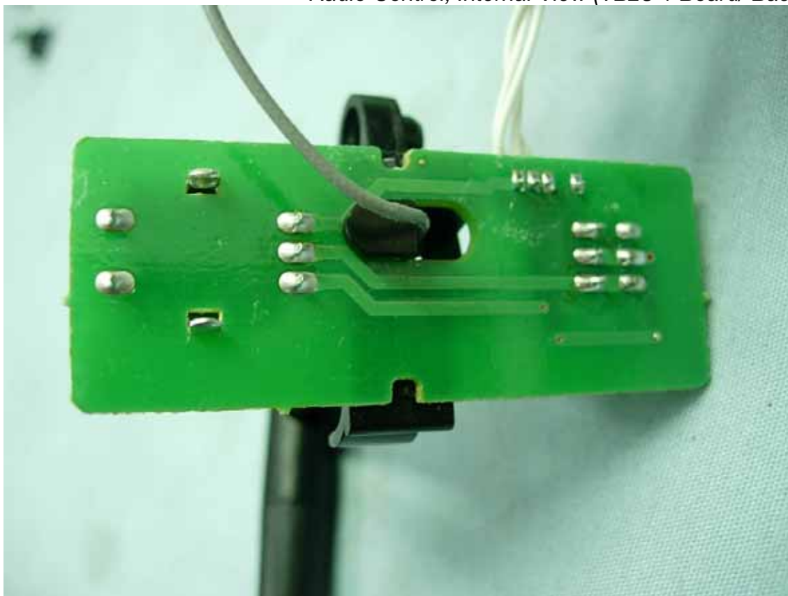
Figure 10 Radio Control, Internal View (TB28-1 Board/ Back View)
