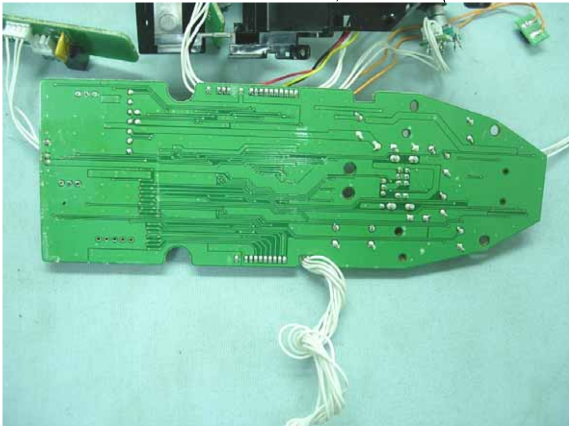
Figure 17 Radio Control, Internal View (Main Board/ Back View)
