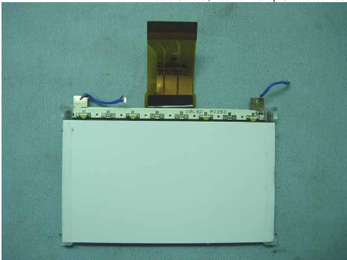
Figure 21 Radio Control, Internal View (LCD Panel/ Back View)
