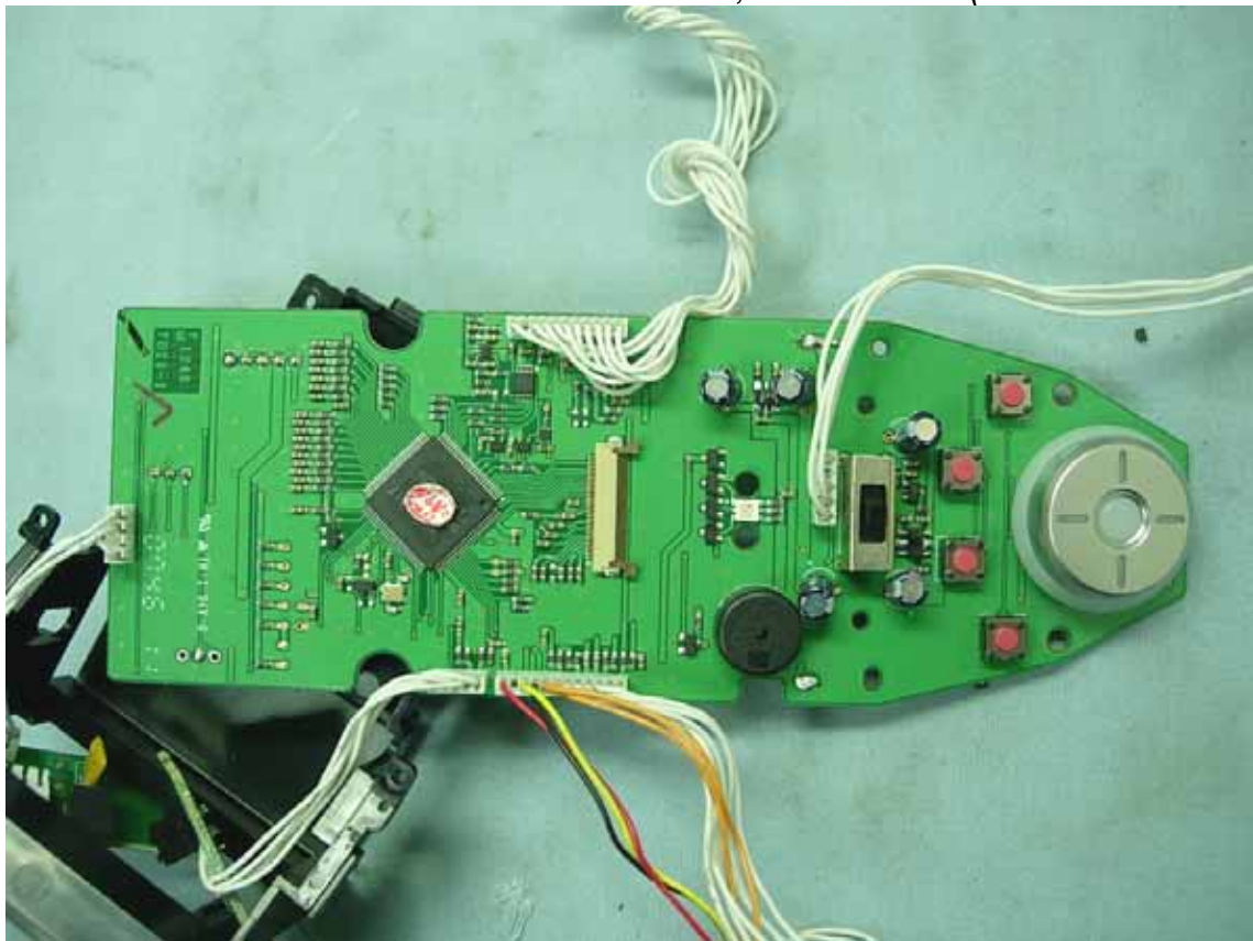
Figure 16 Radio Control, Internal View (Main Board/ Front View)
