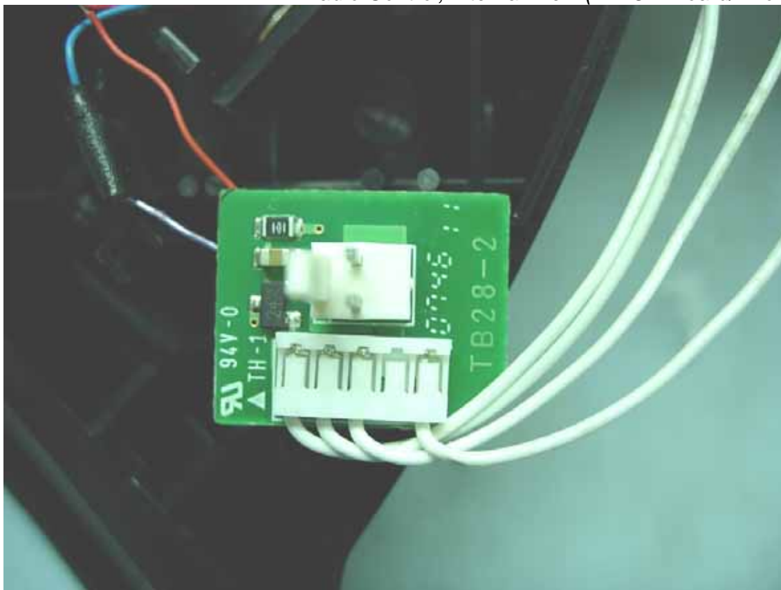
Figure 11 Radio Control, Internal View (TB28-2 Board/ Front View)
