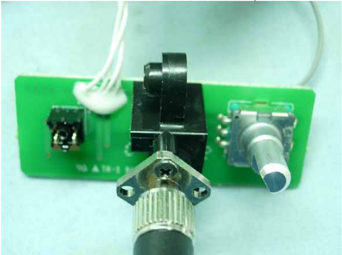
Figure 9 Radio Control, Internal View (TB28-1 Board/ Front View)
