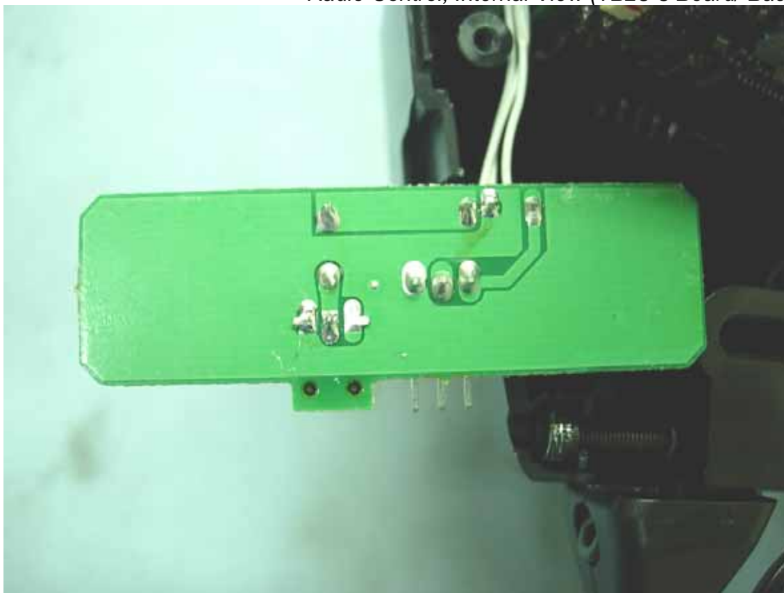
Figure 14 Radio Control, Internal View (TB28-3 Board/ Back View)
