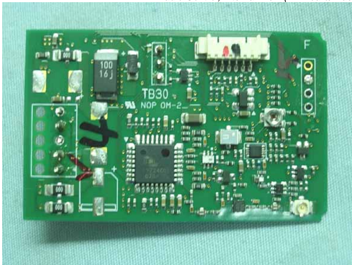
Figure 19 Radio Control, Internal View (RF Board/ Back View)
