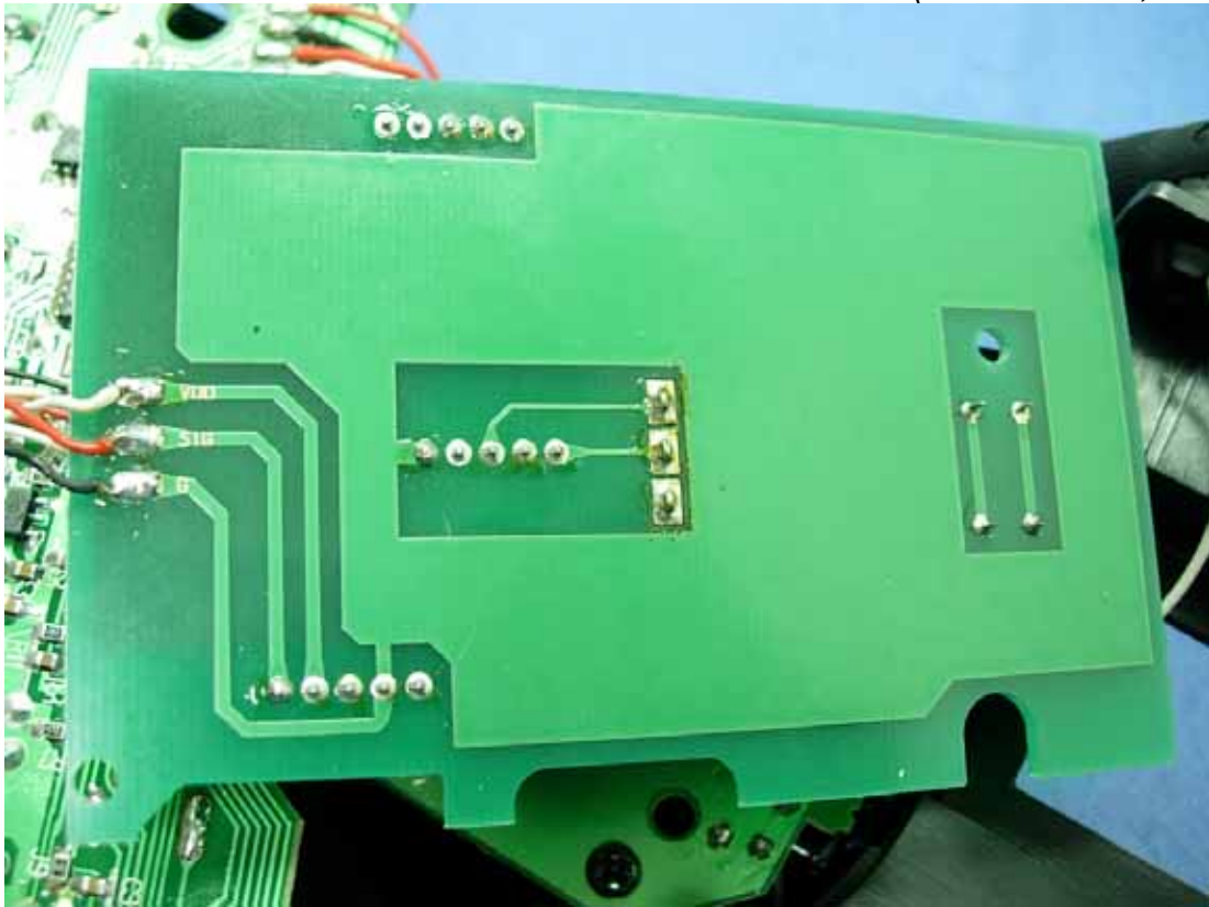
Figure 10 Internal View (Control Board, Back View)
