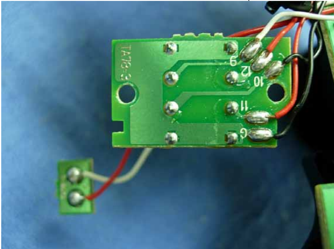
Figure 13 Internal View (Control Boards, Back View)
