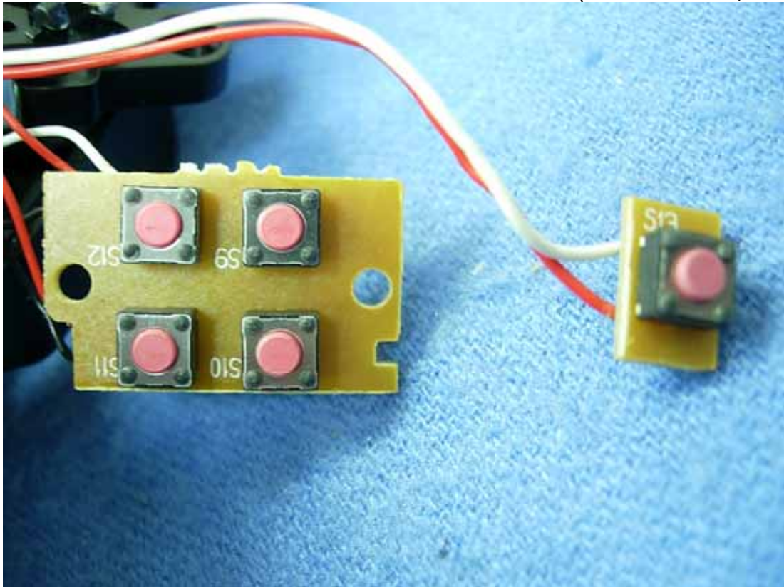
Figure 14 Internal View (Control Boards, Front View)
