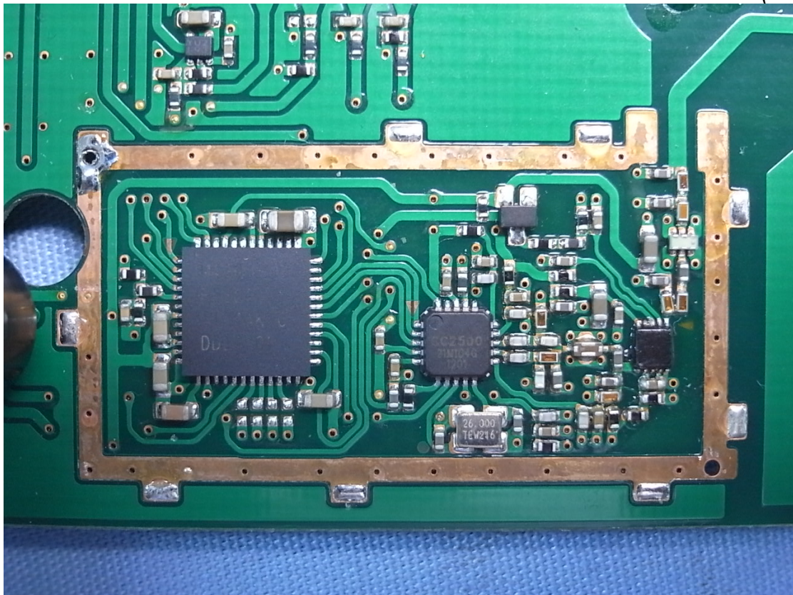
Figure 7 Internal View (RF Board)
