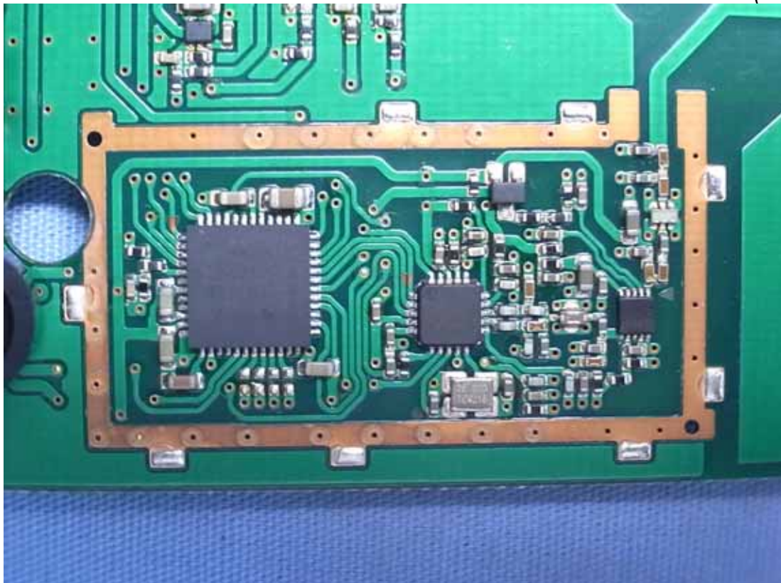
Figure 6 Internal View (RF Board)
