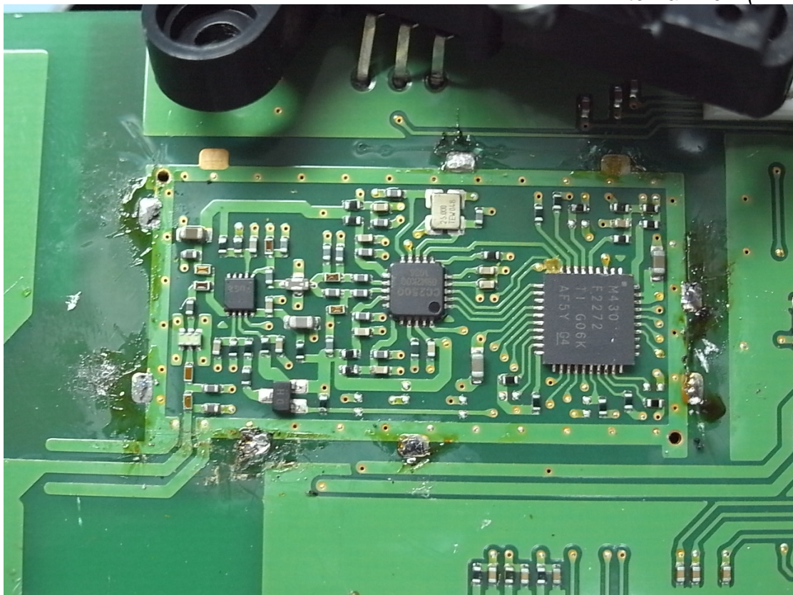
Figure 7 Internal View (RF Module)
