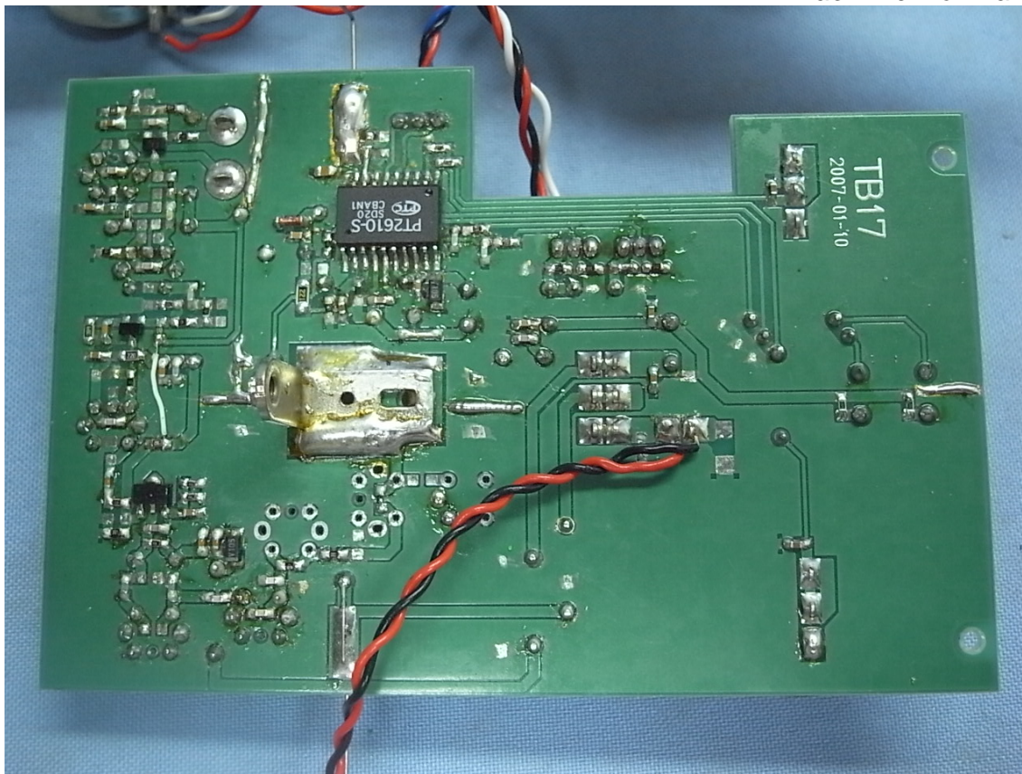
Figure 12 Back View of Main Board
