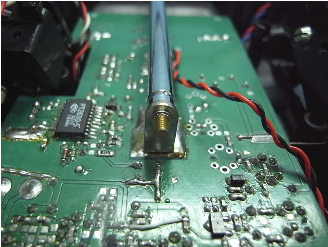
Figure 10 View of 72MHz Crystal
