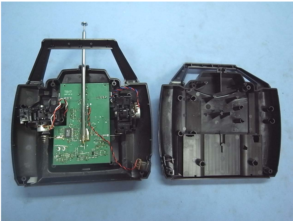
Figure 8 View of Removed Back Cover
