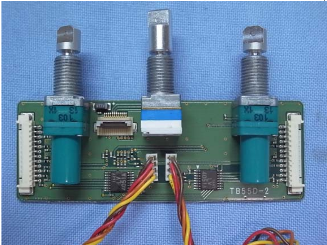
Figure 39 Internal View (TB55D-2 Board, Front View)
