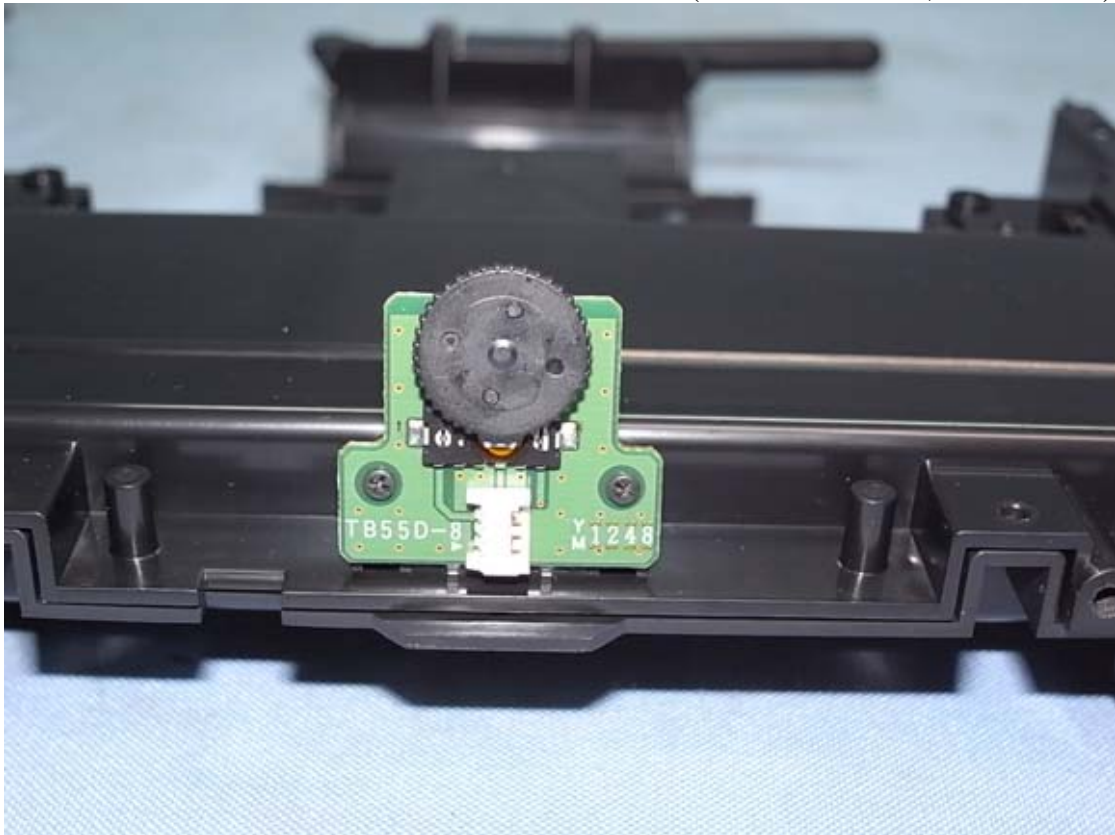
Figure 31 Internal View (TB55D-8 Board, Front View)
