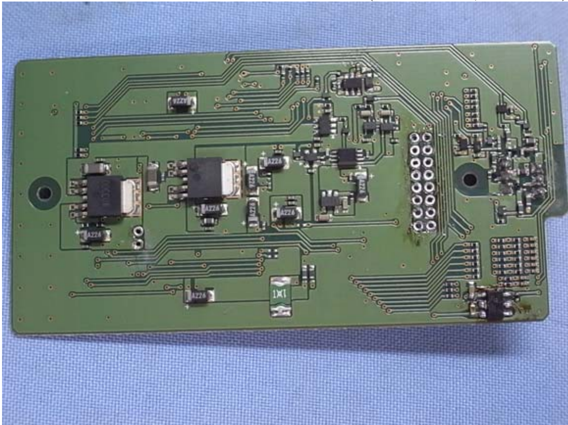
Figure 23 Internal View (TB54D Board, Back View)
