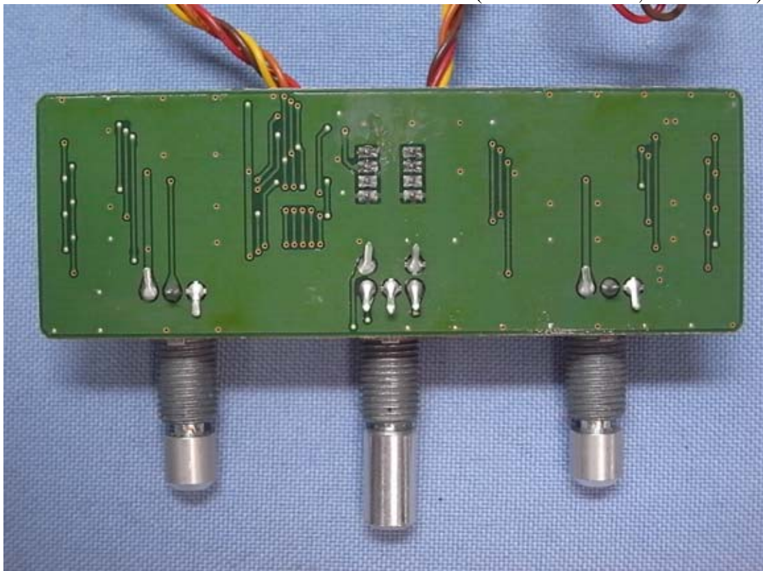
Figure 40 Internal View (TB55D-2 Board, Back View)
