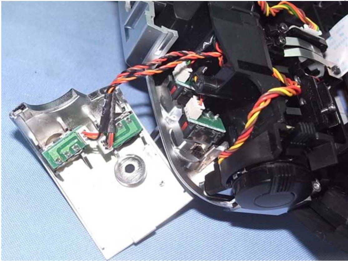
Figure 29 Internal View (Internal Board)
