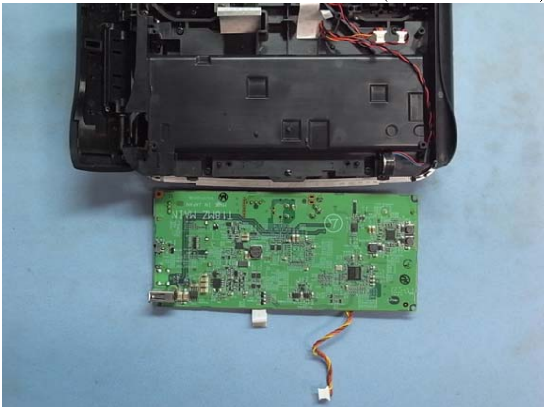
Figure 26 Internal View (Removed Main Board)
