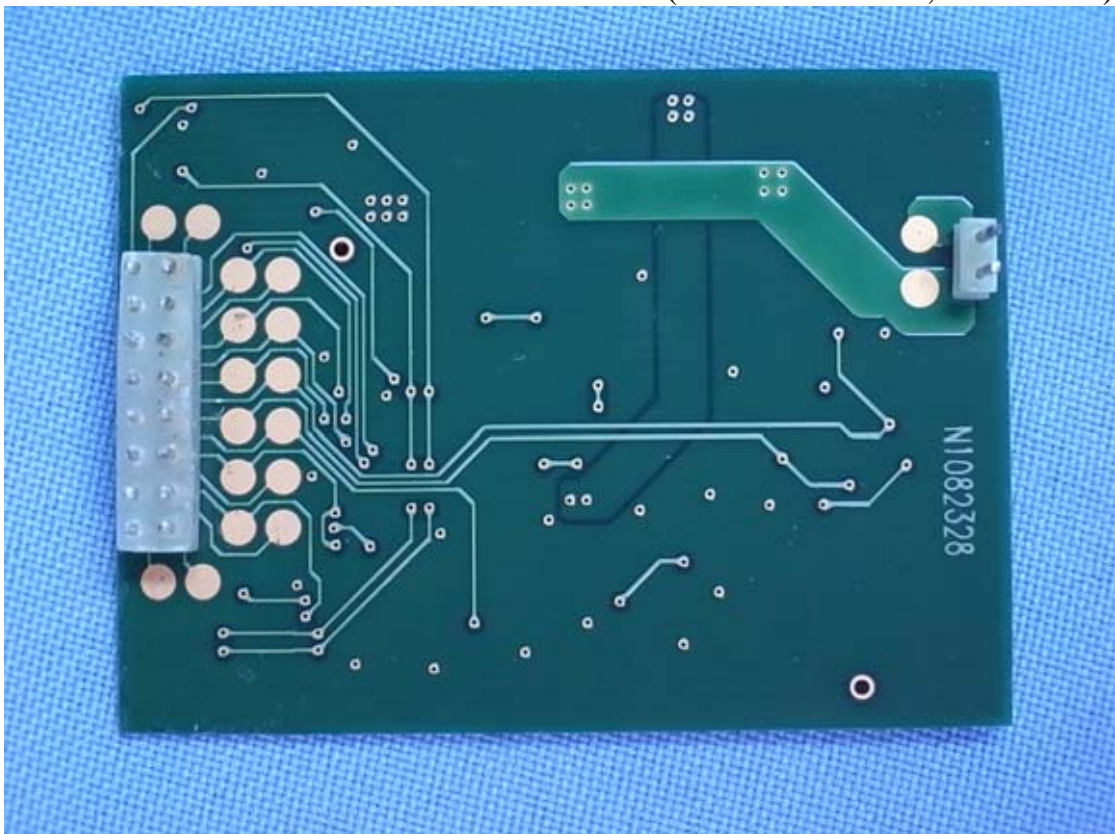
Figure 24 Internal View (TB57A RF Board, Front View)
