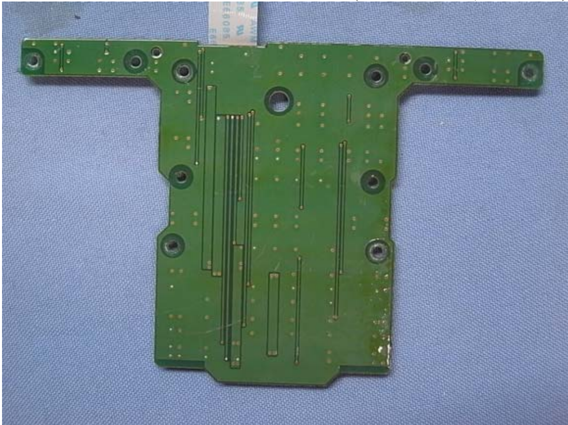
Figure 35 Internal View (TB55D-1 Board, Back View)
