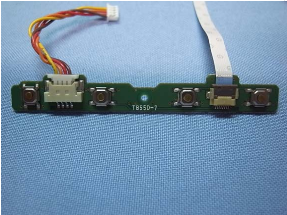
Figure 47 Internal View (TB55D-7 Board, Front View)
