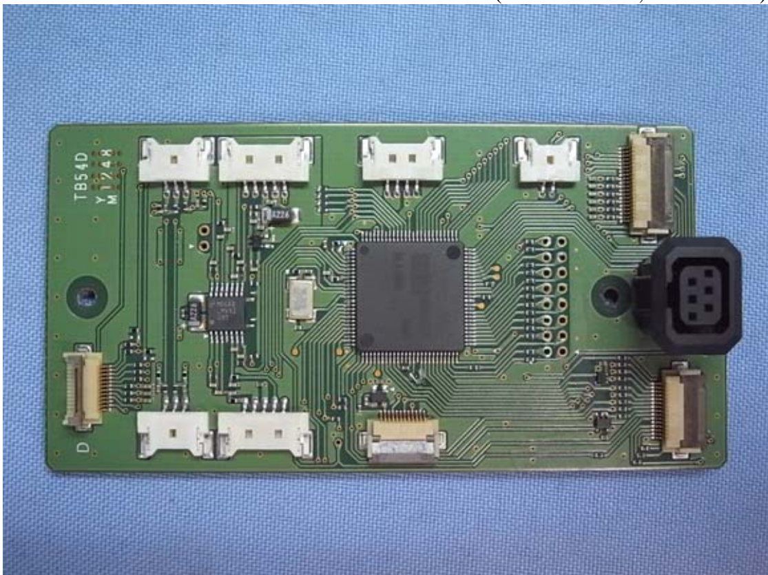
Figure 22 Internal View (TB54D Board, Front View)
