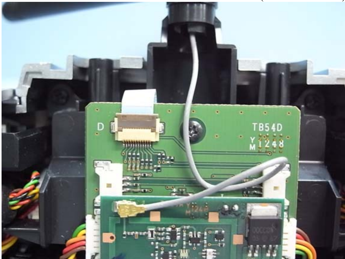
Figure 16 Internal View (RF Antenna View)
