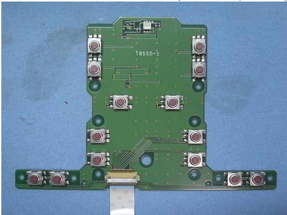
Figure 34 Internal View (TB55D-1 Board, Front View)
