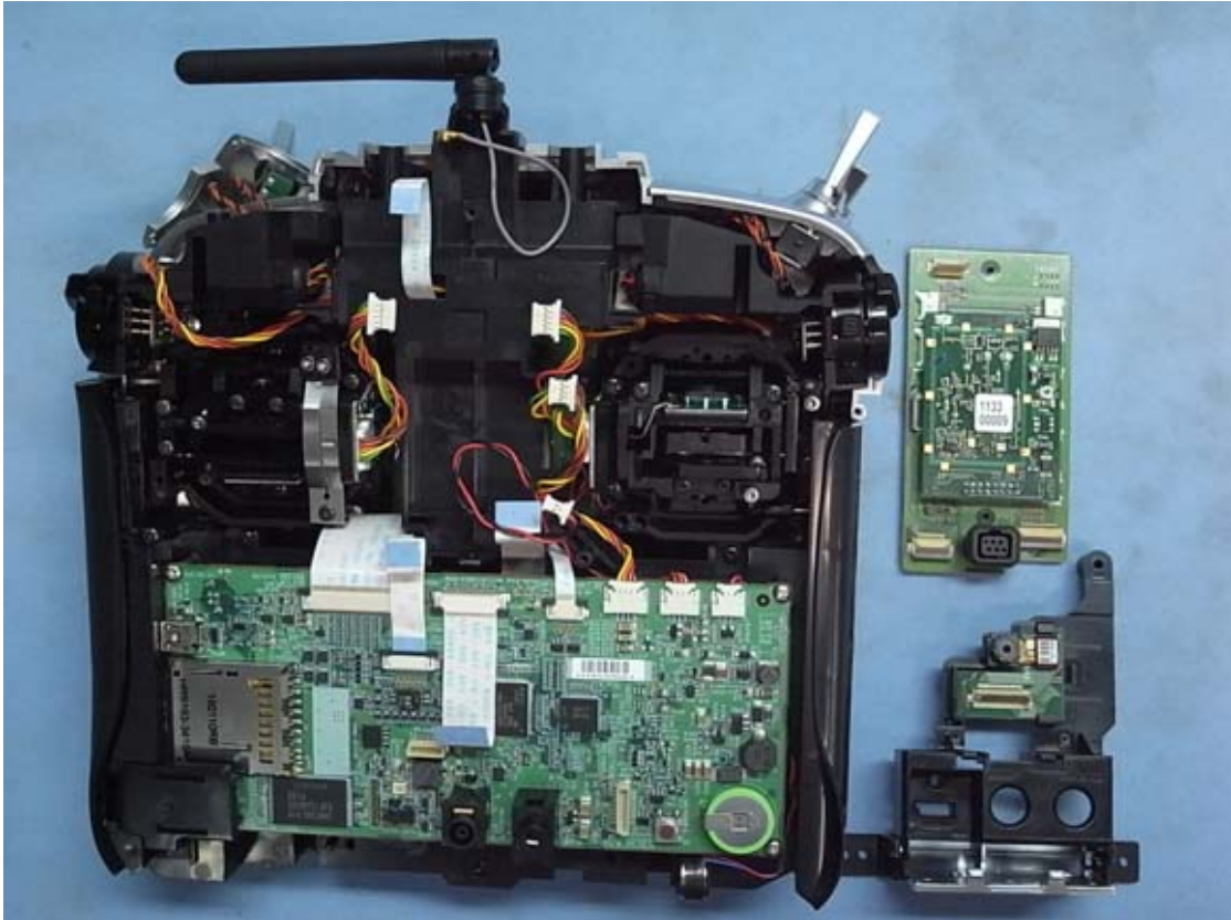
Figure 17 Internal View (Removed PCB)
