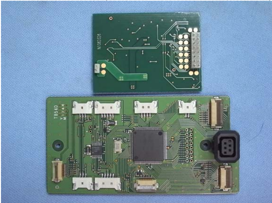
Figure 21 Internal View (TB57A RF Board & TB54D Board, Back View)
