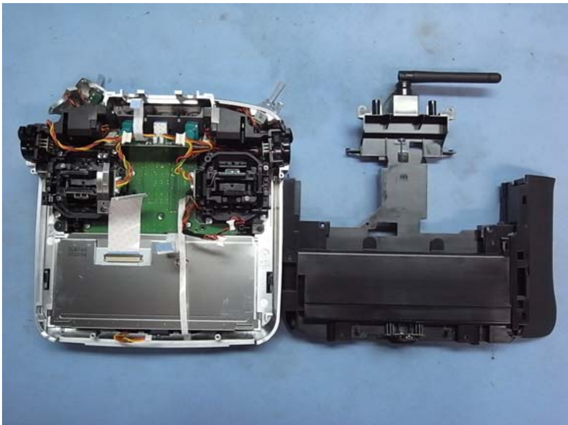
Figure 30 Internal View
