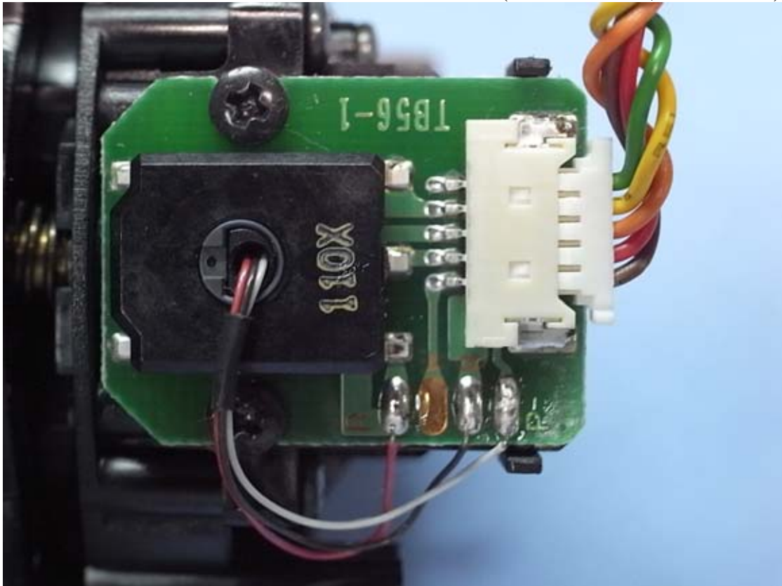
Figure 37 Internal View (TB56-1 Board, Front View)
