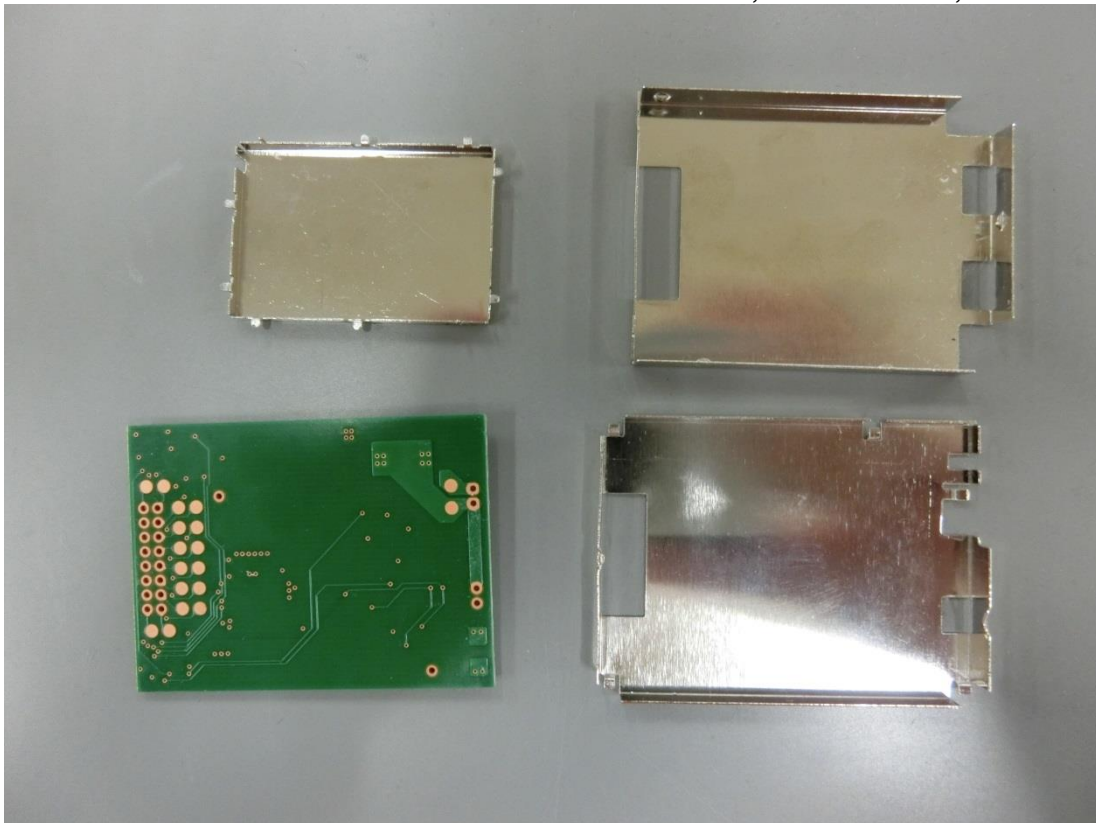
Figure 28 Wireless Module, Internal View, Back View
