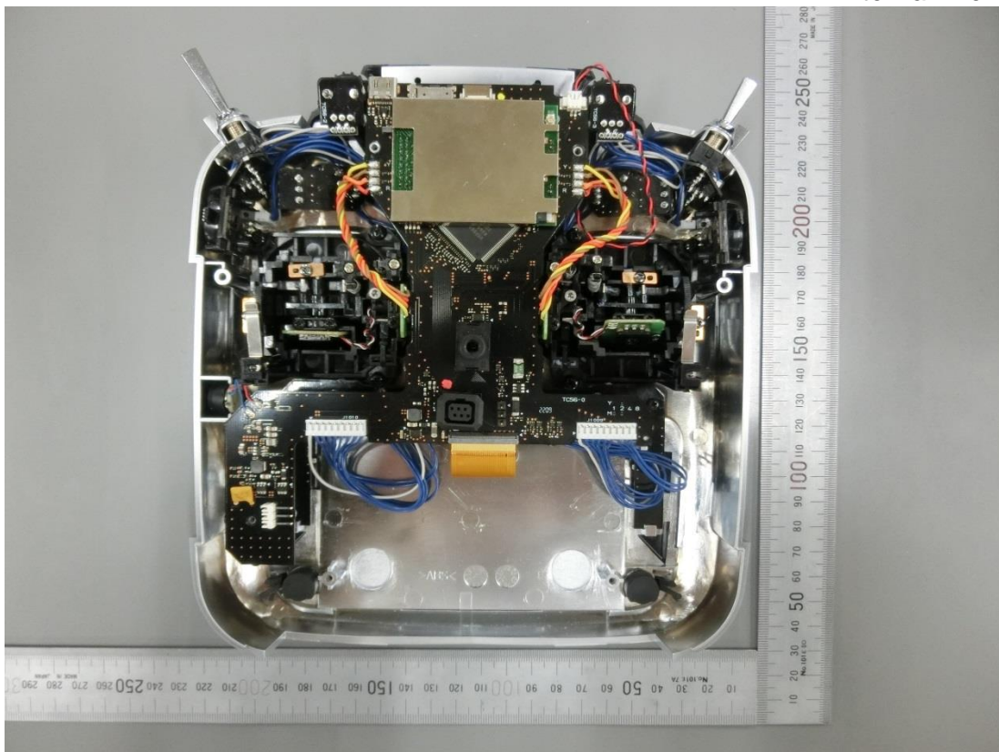
Figure 16 Internal View
