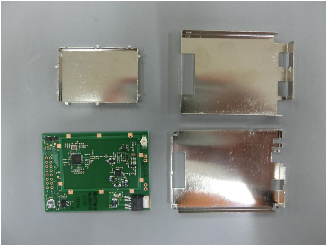
Figure 27 Wireless Module, Internal View, Front View
