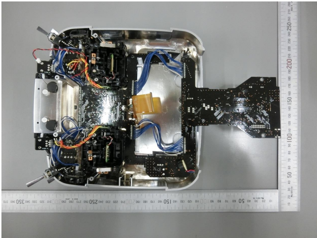
Figure 17 Internal View
