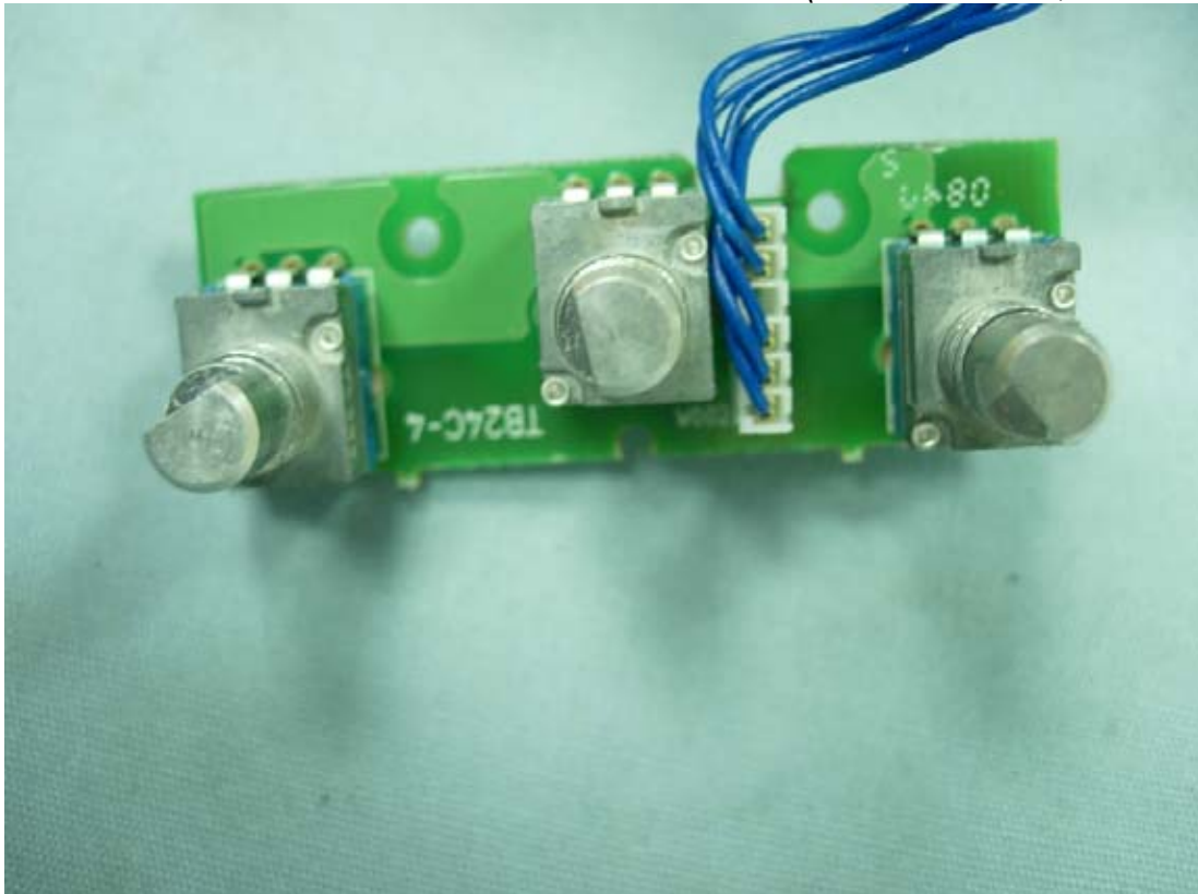
Figure 25 Internal View (TB24C-4 Board, Front View)
