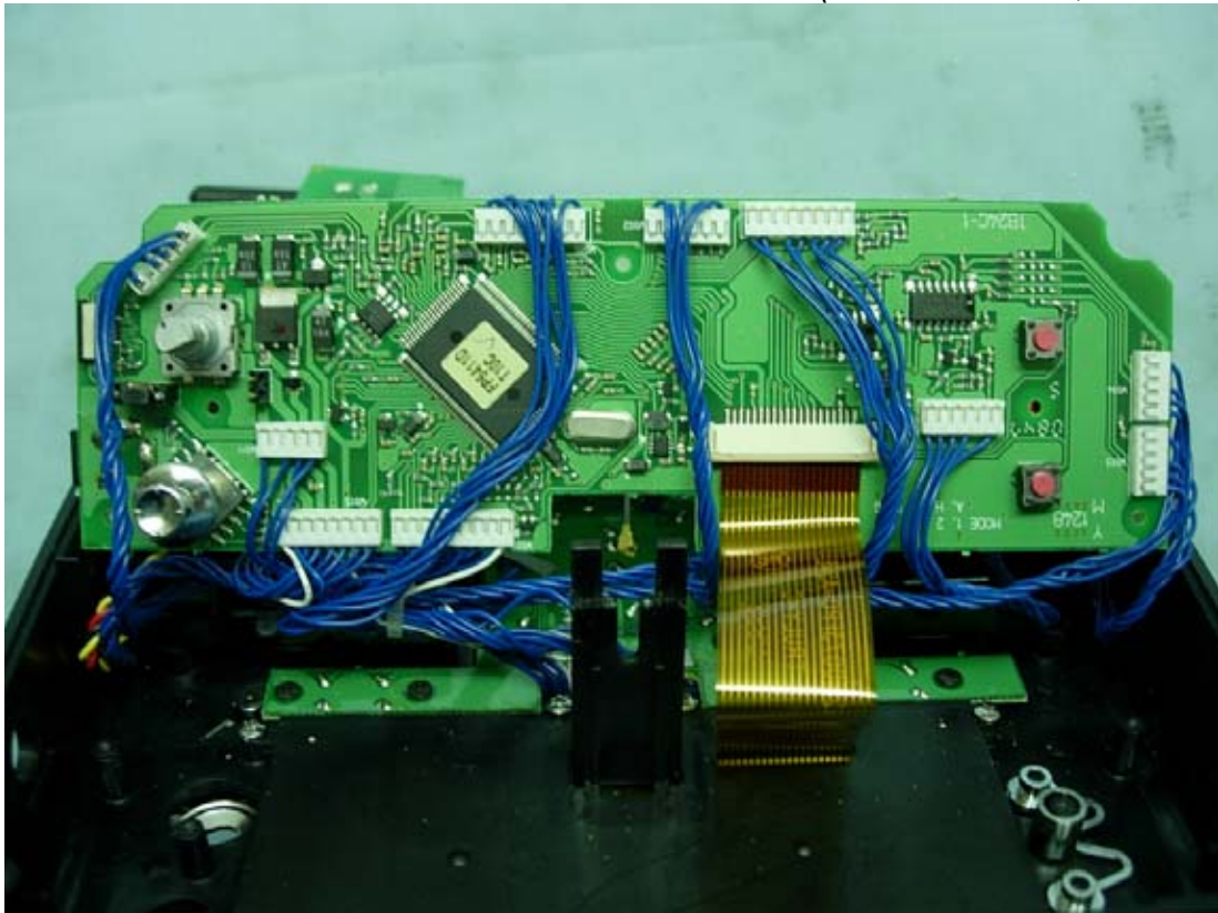
Figure 17 Internal View (TB24C-1 Board, Front View)
