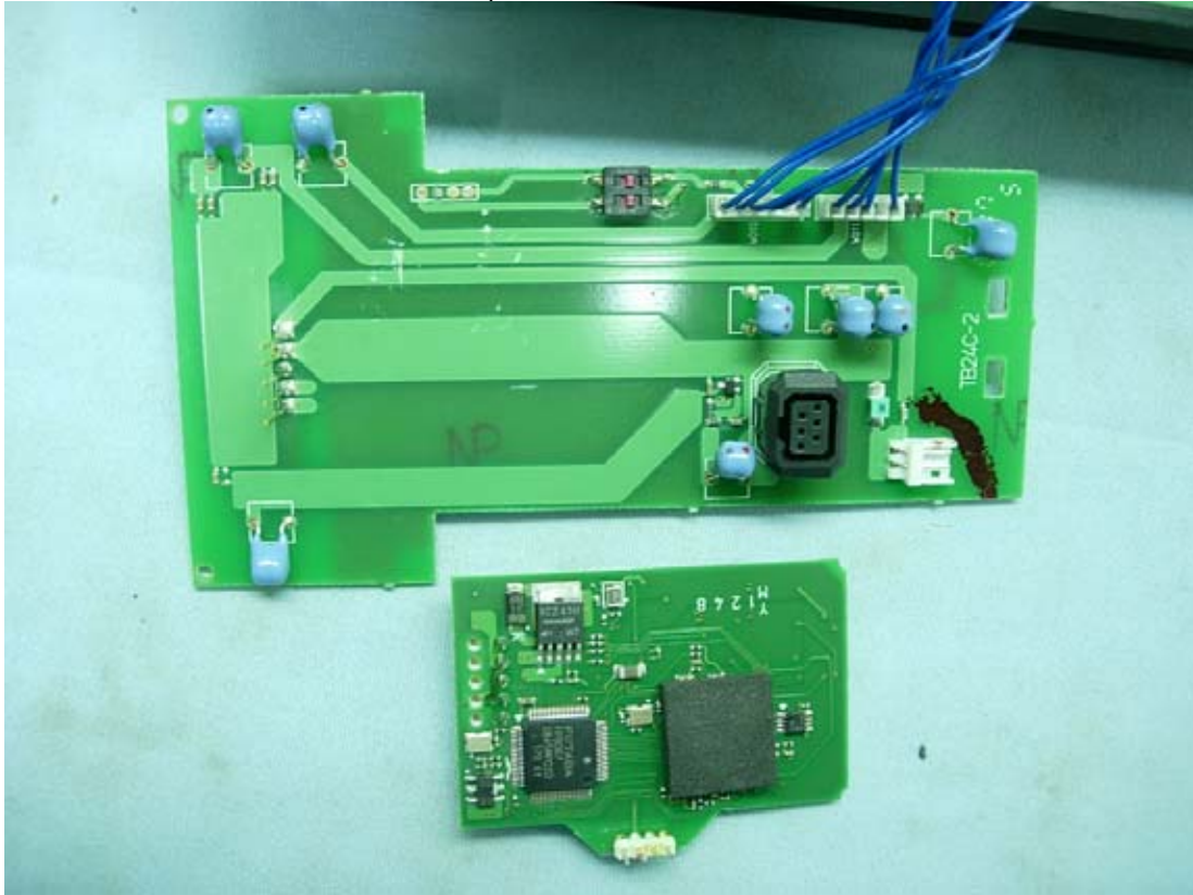
Figure 12 Internal View (Removed RF Board, TB24C-2 Board/Front View)
