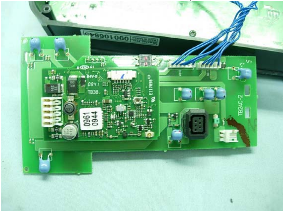
Figure 11 Internal View (TB24C-2 Board & RF Board)
