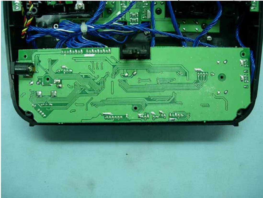
Figure 16 Internal View (TB24C-1 Board, Back View)
