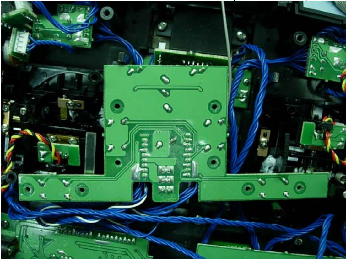
Figure 20 Internal View (TB24C-3 Board, Back View)
