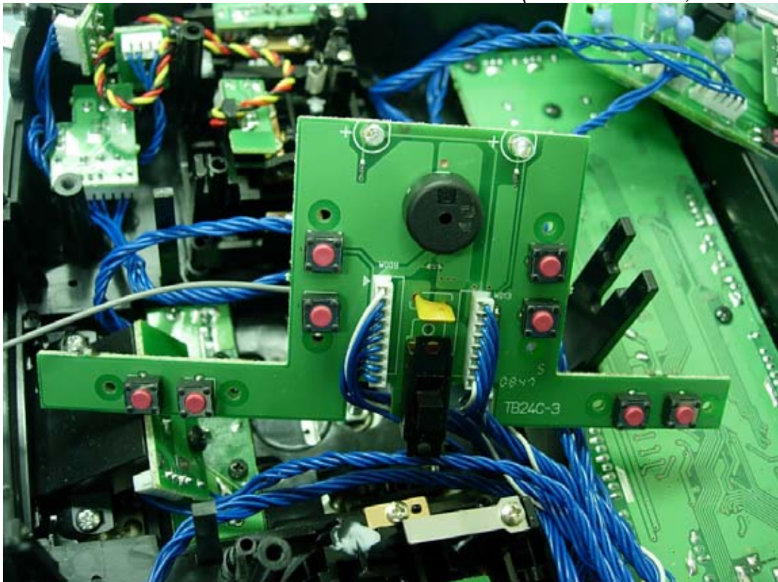
Figure 21 Internal View (TB24C-3 Board, Front View)
