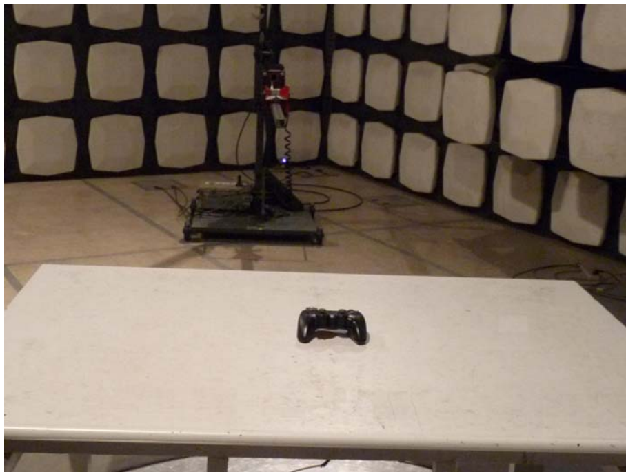
Figure 2 Test photo of Transmitter Spurious Emission (TX Mode 1000-25000MHz)
