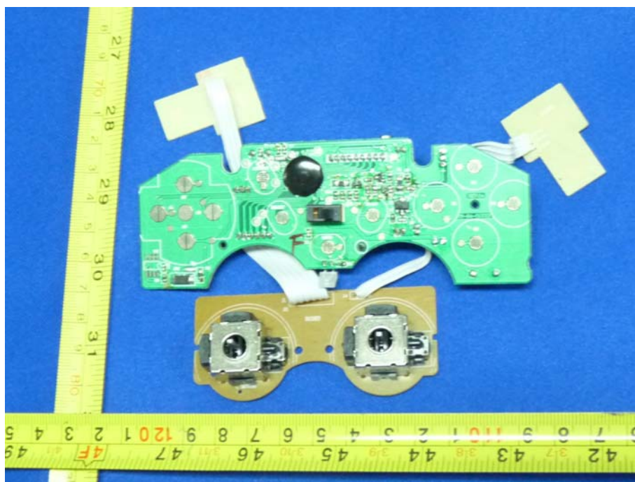
Figure 2 Internal photo of PCB
