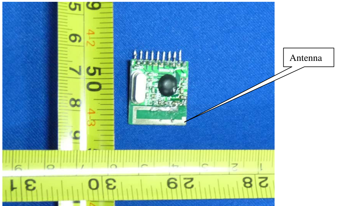
Figure 3 Internal photo of PCB
