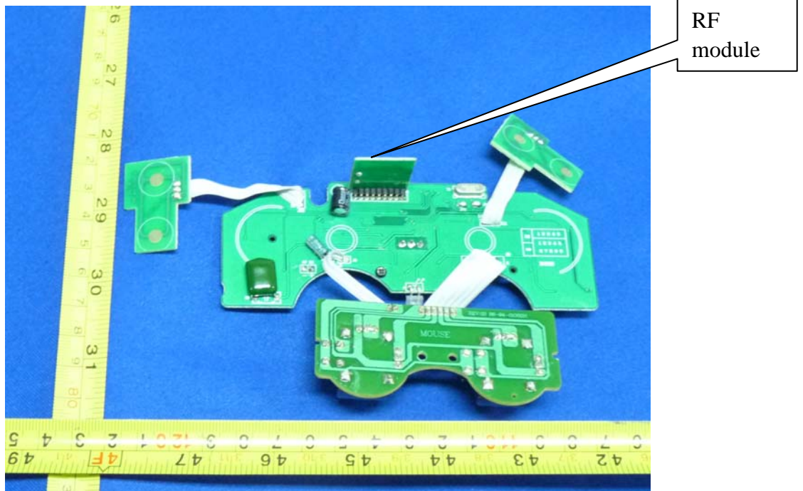
Figure 1 Internal photo of PCB
