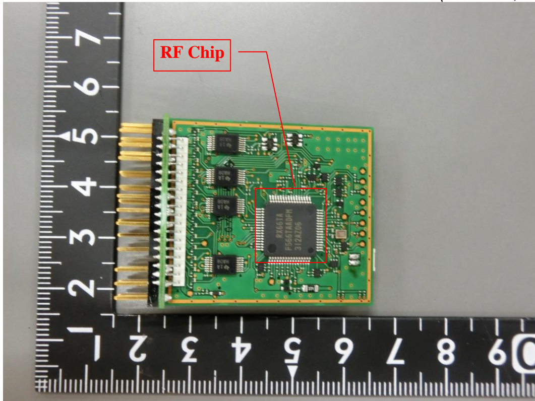
Internal View (RF Board, Front View)
