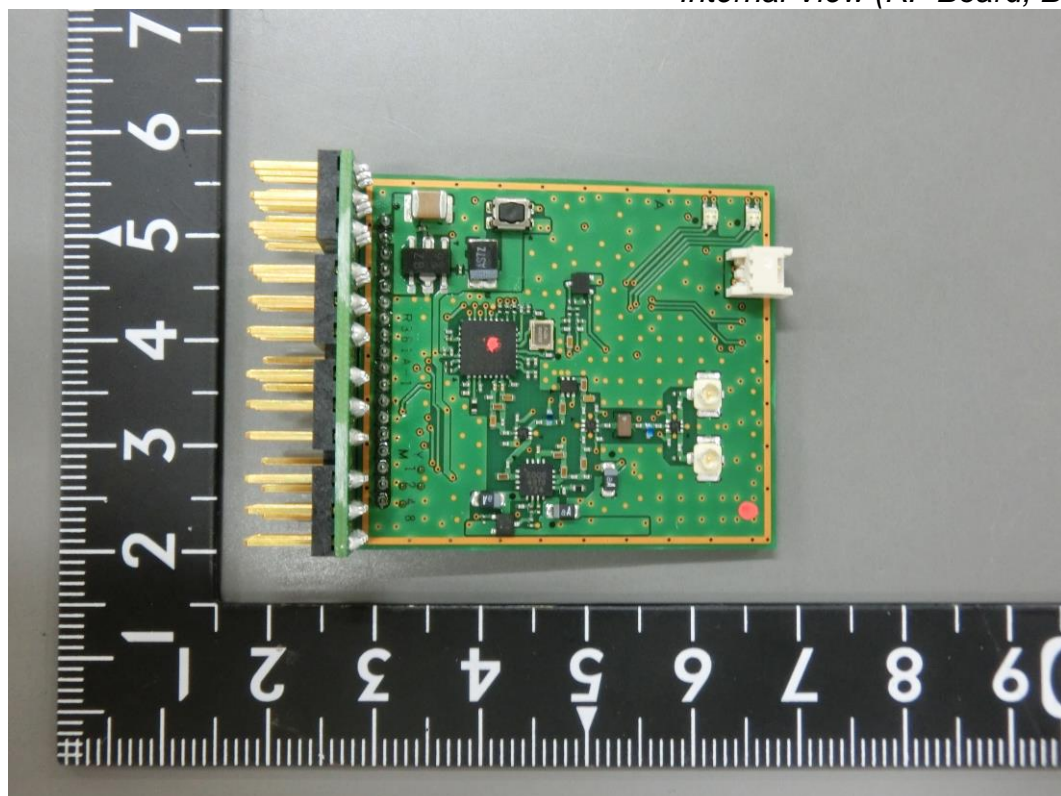
Internal View (RF Board, Back View)
