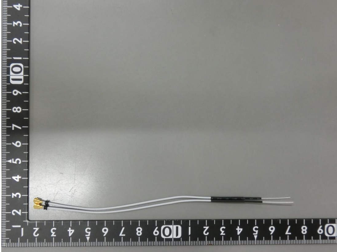
Figure 4 General Appearance (U.FL-LP-068N1T-21-(120)D Antenna)
