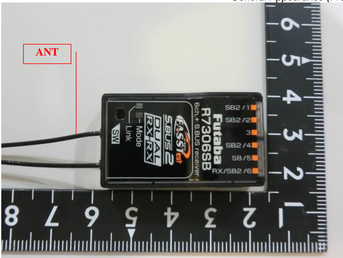
Figure 8 General Appearance (Front View)
