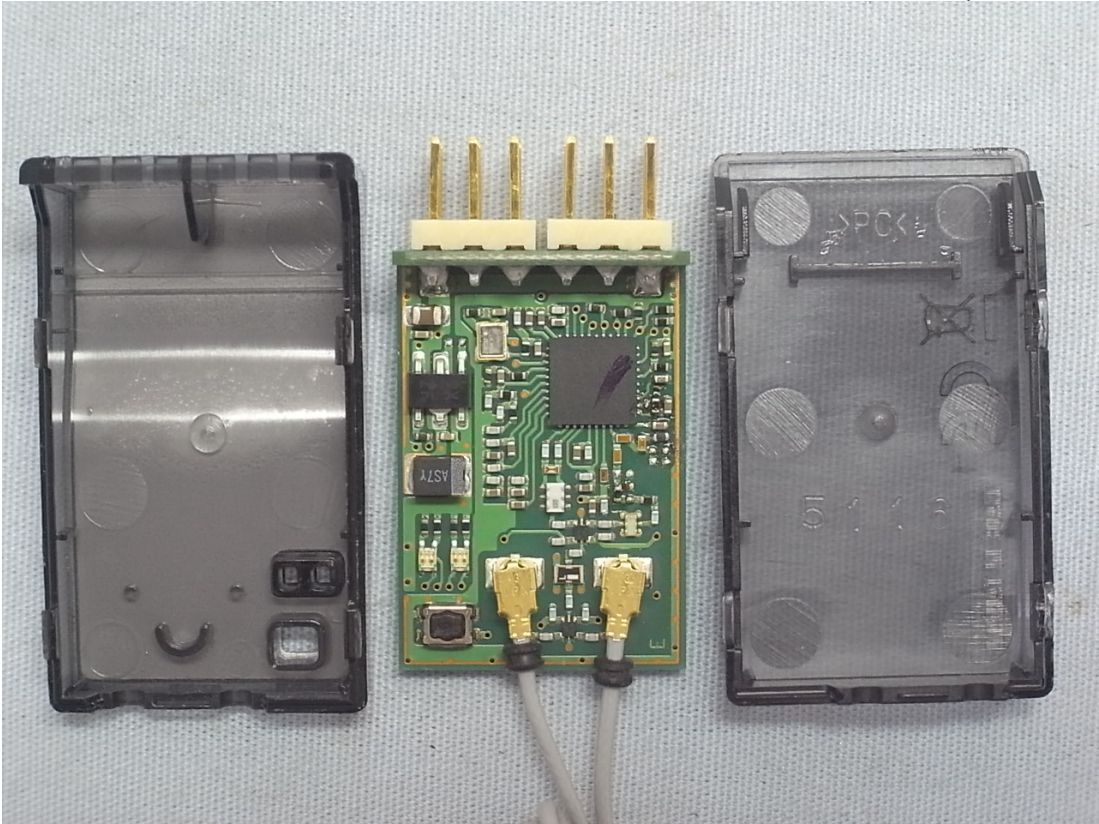
Figure 4 Internal View (RF Board, Front View)
