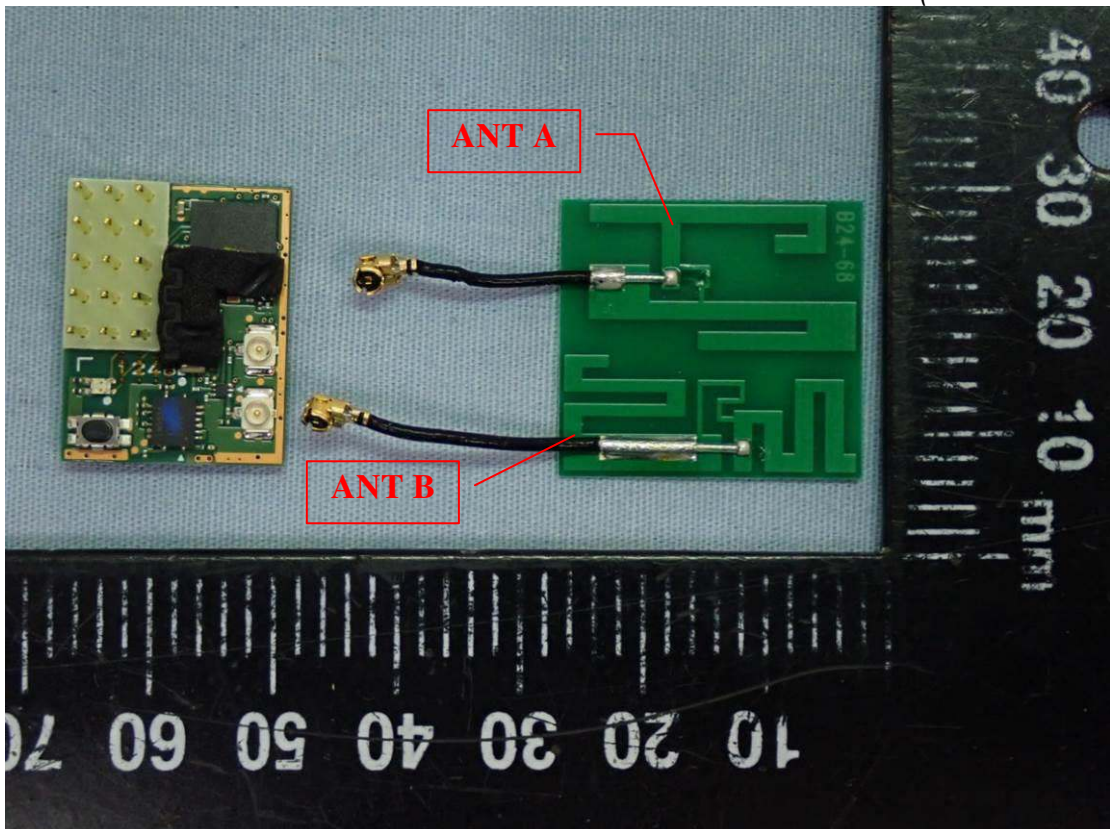
Internal View (Removed RF Board)
