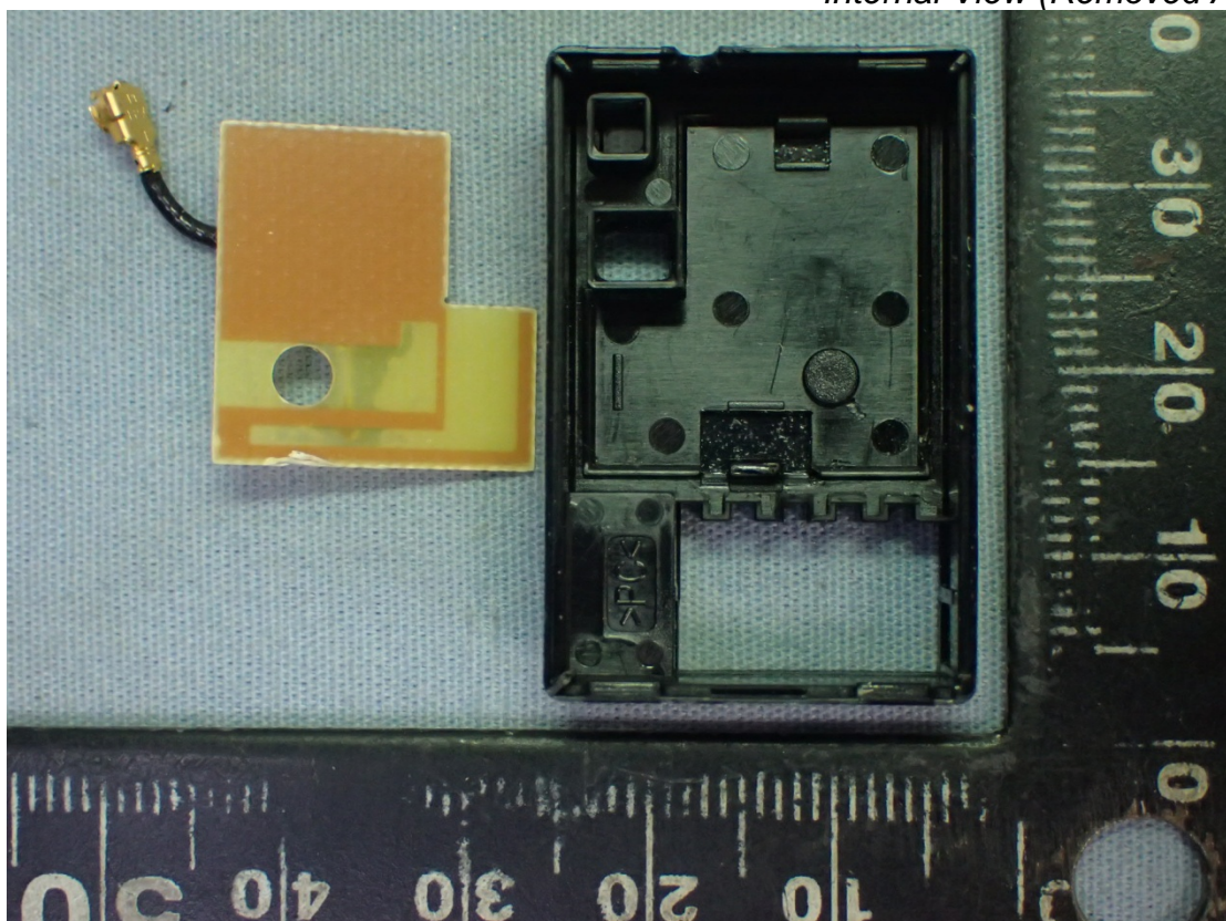
Internal View (Removed Antenna)
