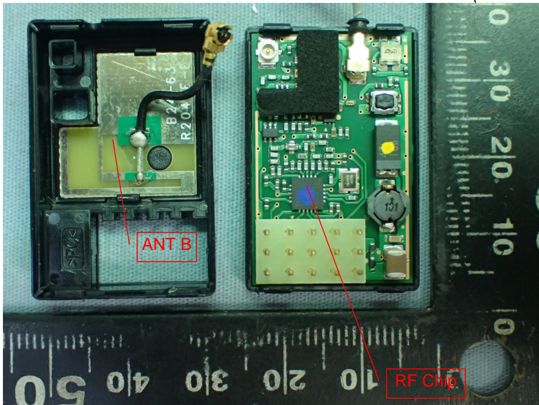
Internal View (Removed Cover)
