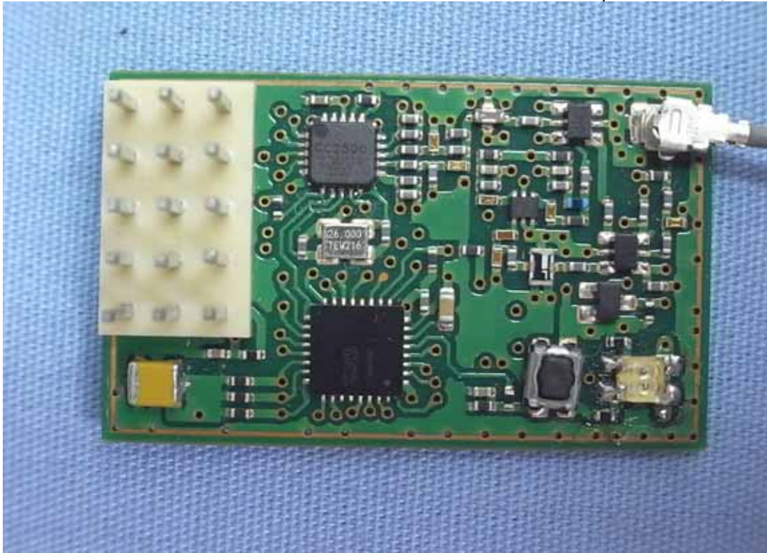
Figure 4 Internal View (Main Board, Front View)
