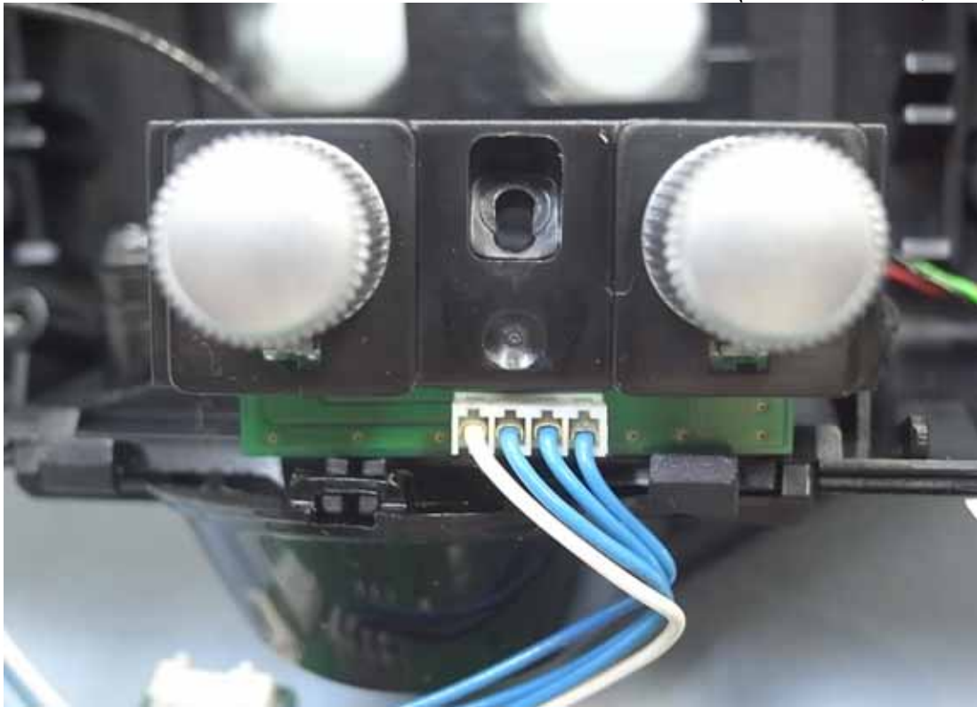
Figure 25 Internal View (Control Board, Front View)
