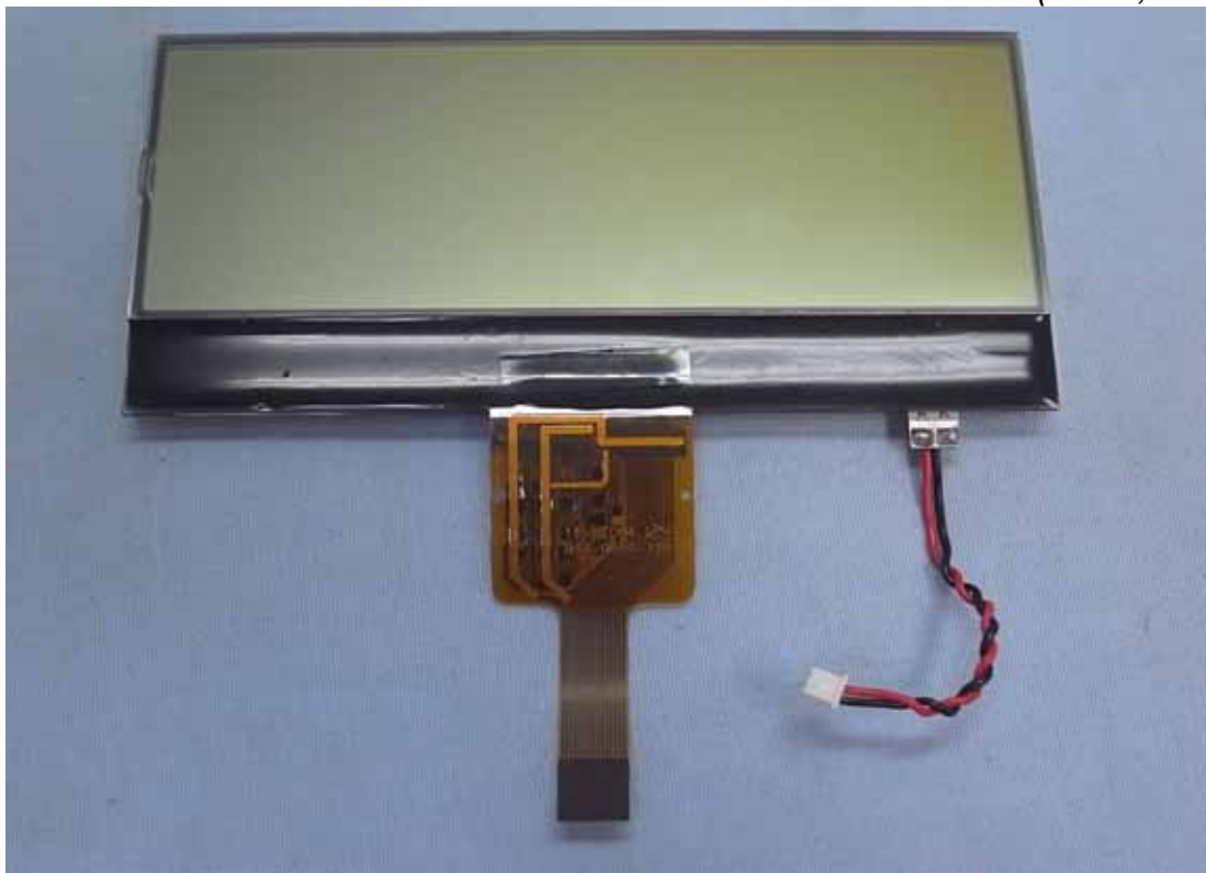
Figure 11 Internal View (Panel, Front View)
