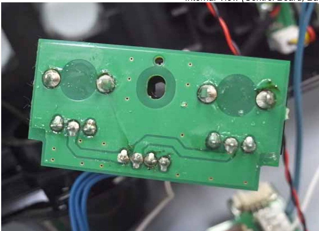
Figure 26 Internal View (Control Board, Back View)
