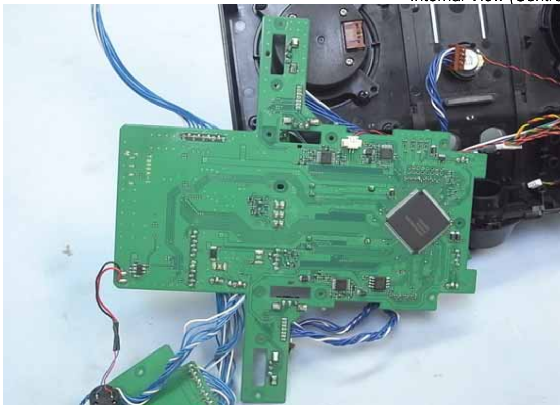
Figure 22 Internal View (Control Board)
