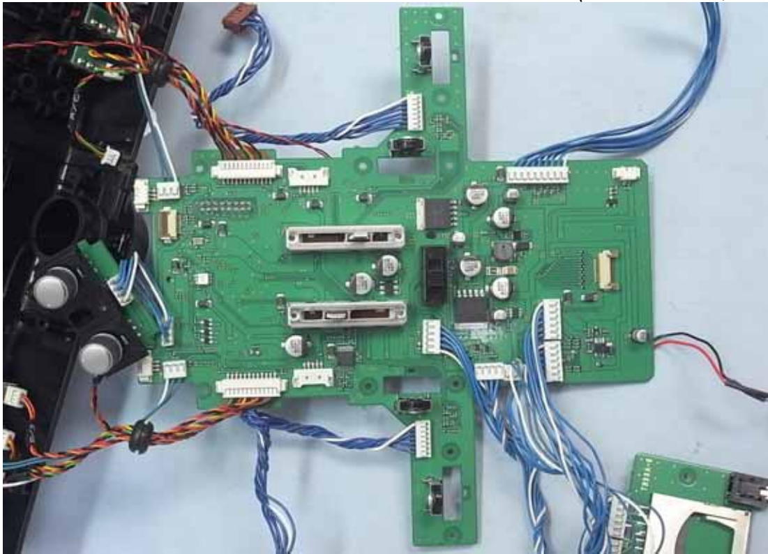
Figure 19 Internal View (Control Board, Front View)
