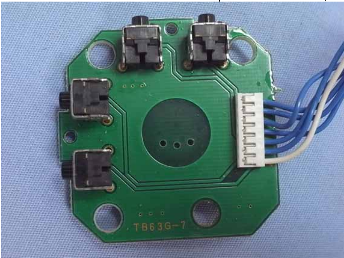
Figure 12 Internal View (Function Control Board, Front View)
