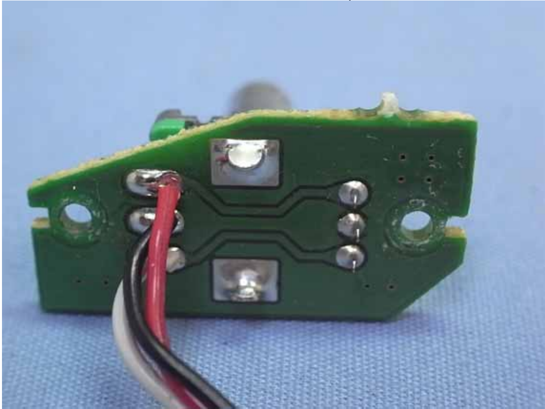
Figure 15 Internal View (Function Control Board, Back View)
