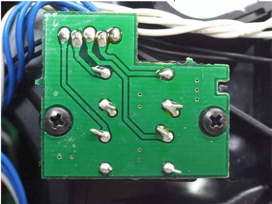
Figure 10 Internal View (Function Control Board, Back View)
