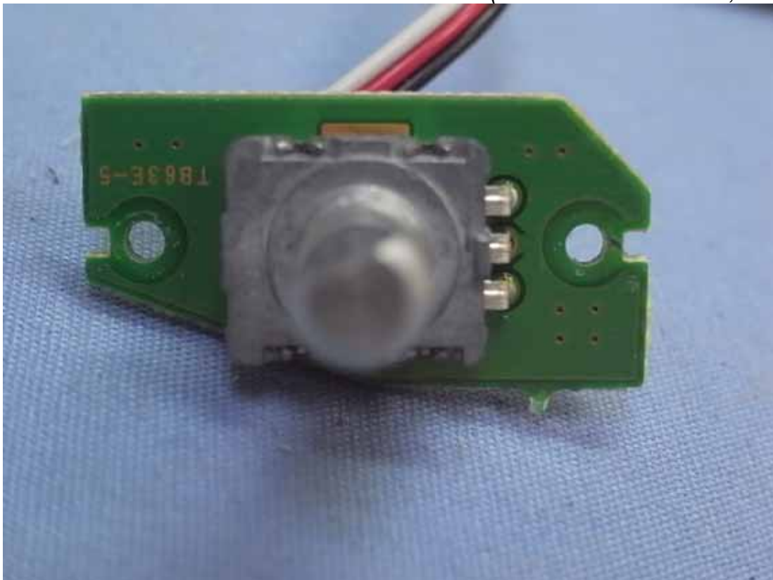
Figure 14 Internal View (Function Control Board, Front View)
