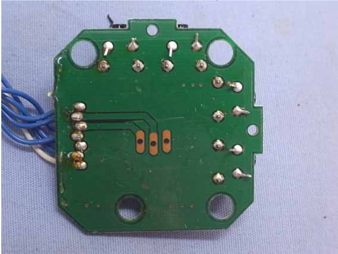
Figure 13 Internal View (Function Control Board, Back View)
