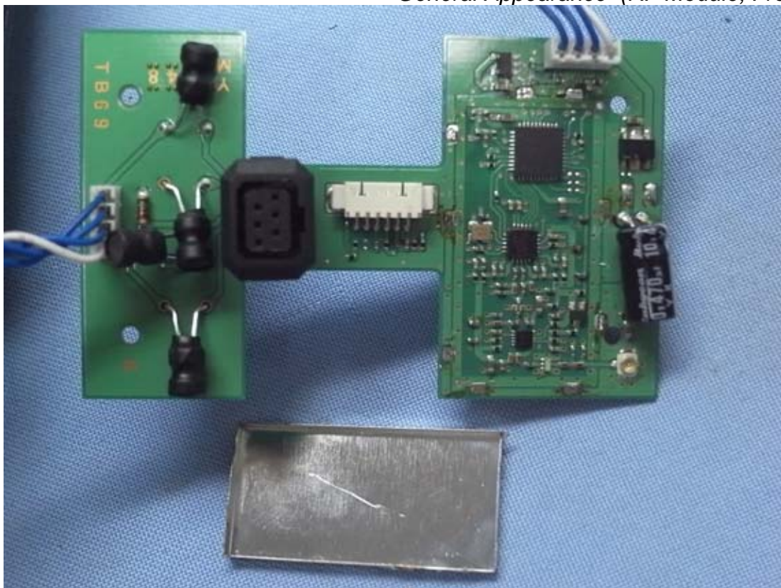
Figure 6 General Appearance (RF Module, Front View)
