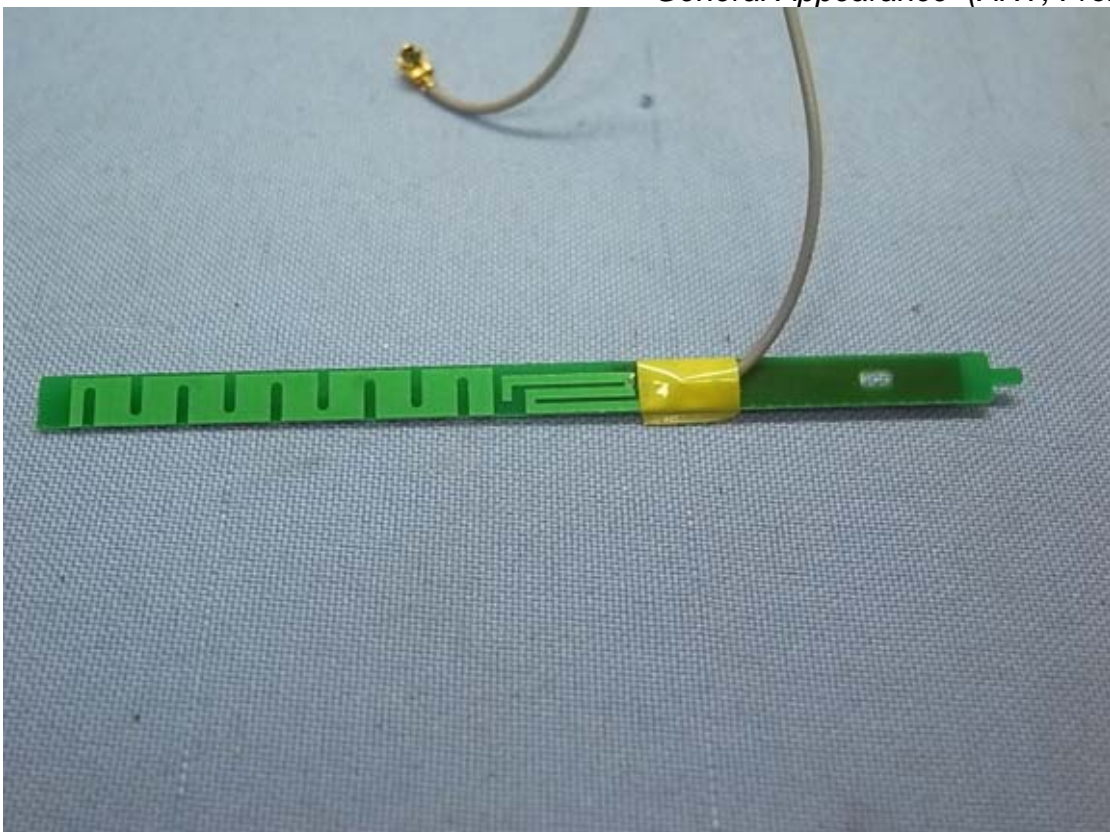
Figure 8 General Appearance (ANT, Front View)
