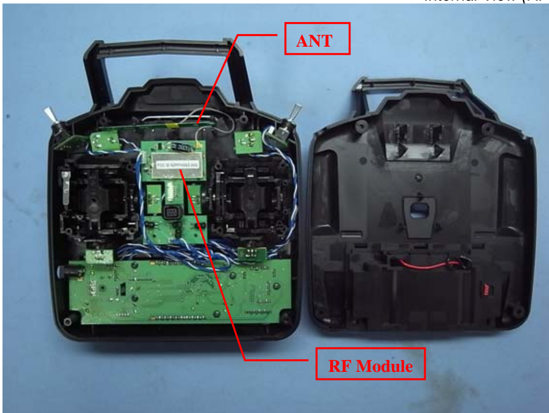
Figure 4 Internal View (RF Module)
